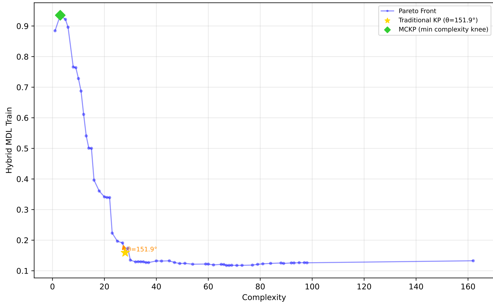
227_cpu_small - Run 6 - MVP - Hybrid MDL Train \lambda_1=0.80, \lambda_2=0.20, \lambda_3=0.00 | Difficulty: 1.00 | Method: hmr
