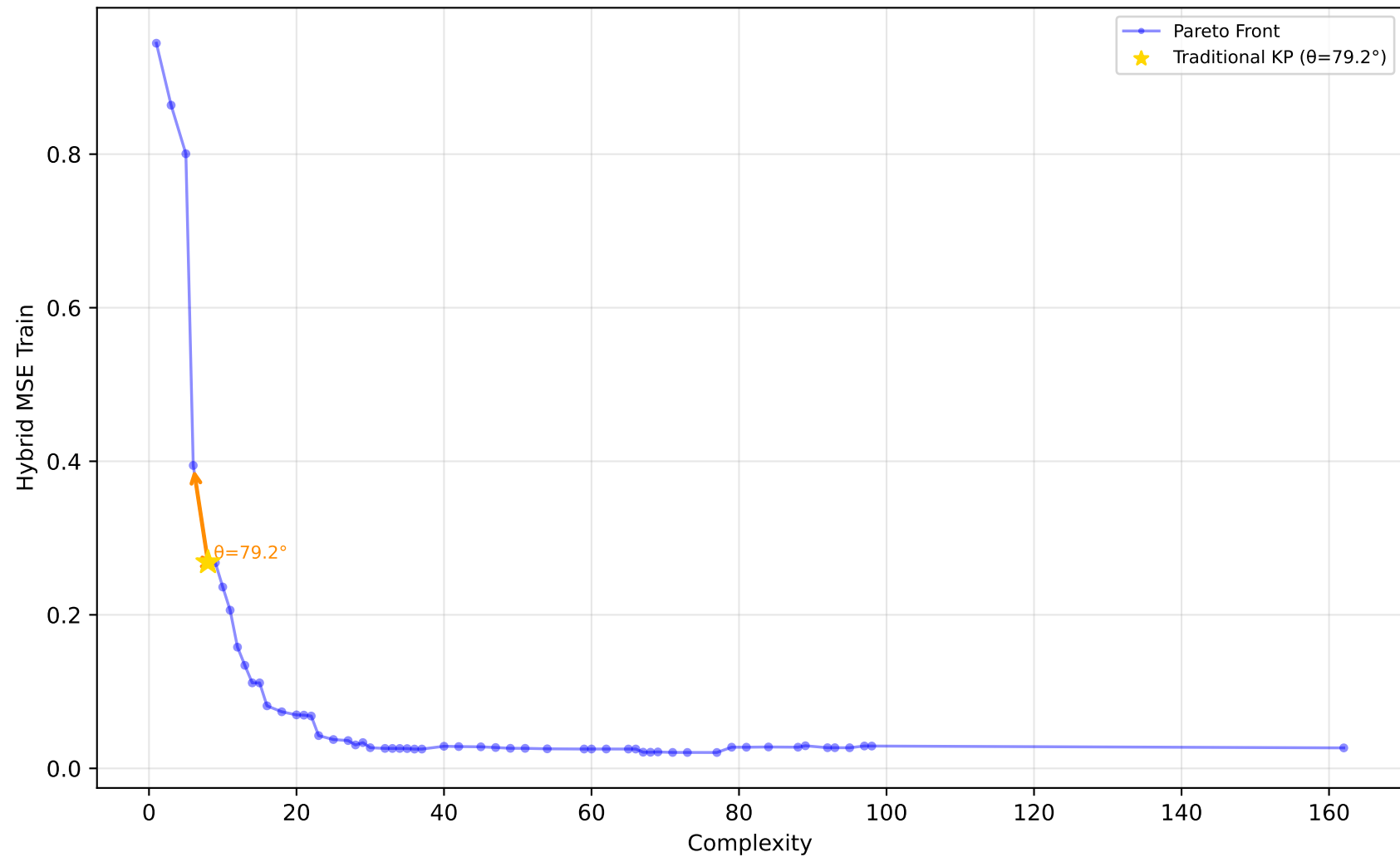
227_cpu_small - Run 6 - MVP - Hybrid MSE Train \lambda_1=0.00, \bar{\lambda}_2=0.90, \lambda_3=0.10 | Difficulty: 1.00 | Method: hmr
