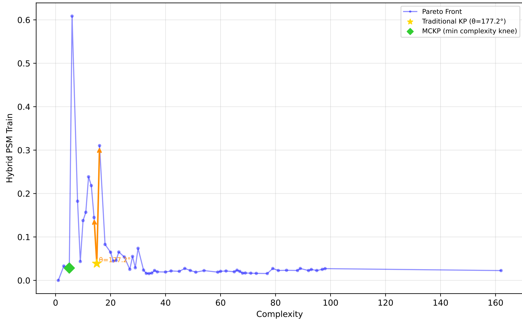
227_cpu_small - Run 6 - MVP - Hybrid PSM Train \lambda_1=0.00, \bar{\lambda}_2=0.90, \lambda_3=0.10 | Difficulty: 1.00 | Method: hmr
