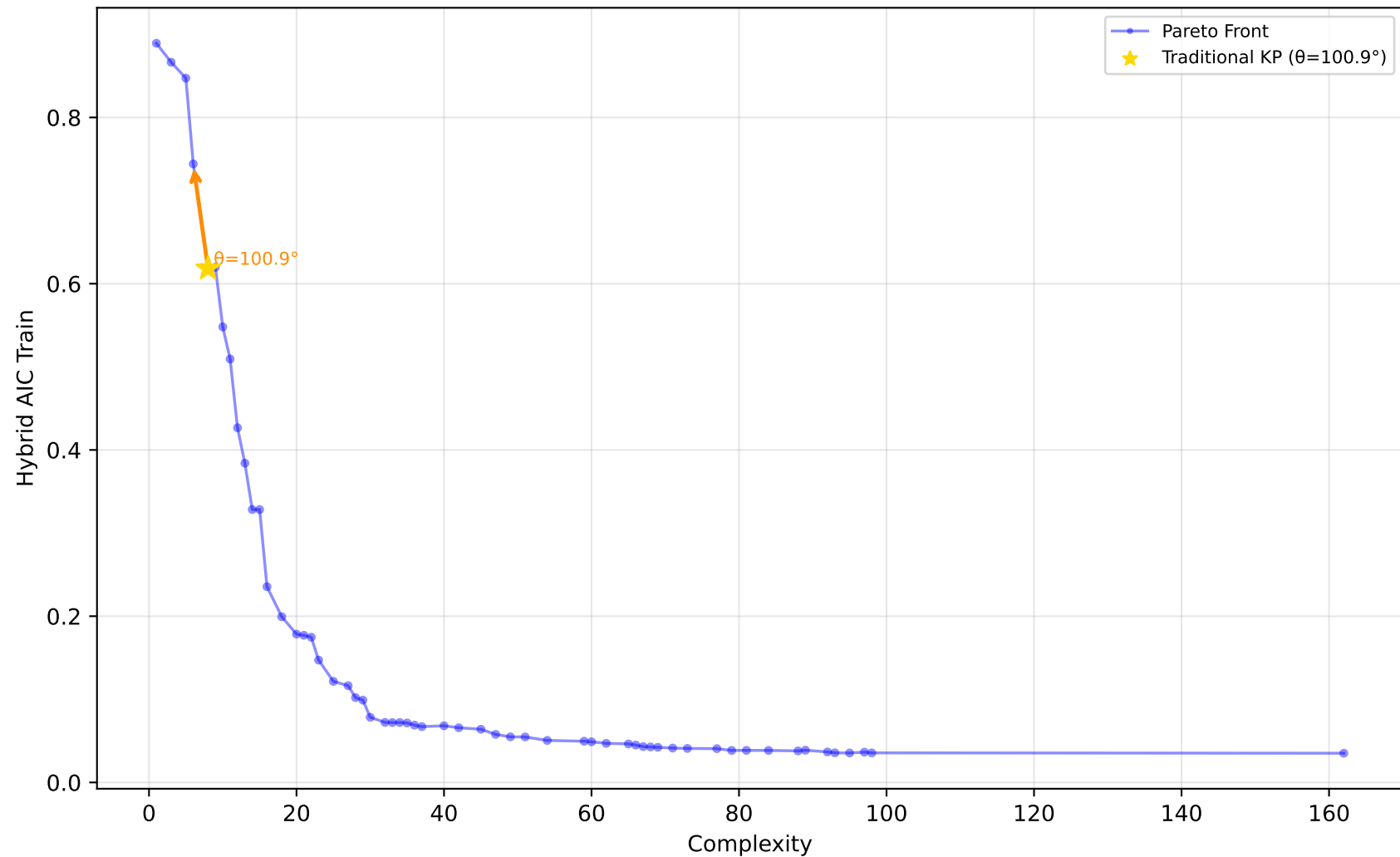
227_cpu_small - Run 6 - SVP - Hybrid AIC Train \lambda_1=0.00, \lambda_2=0.80, \lambda_3=0.30 | Difficulty: 1.00 | Method: hmr
