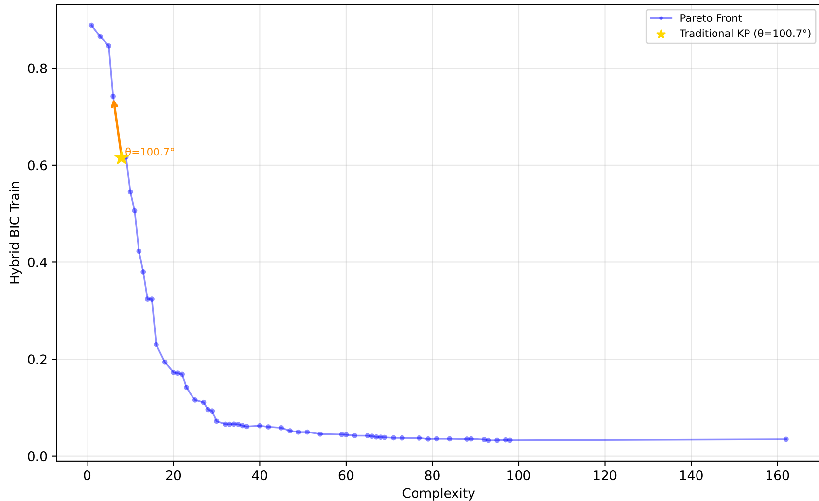
227_cpu_small - Run 6 - SVP - Hybrid BIC Train \lambda_1=0.00, \lambda_2=0.80, \lambda_3=0.30 | Difficulty: 1.00 | Method: hmr
