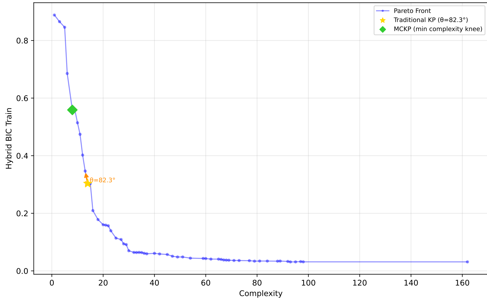
227_cpu_small - Run 6 - SVP - Hybrid BIC Train \lambda_1=0.00, \lambda_2=1.00, \lambda_3=0.00 | Difficulty: 1.00 | Method: hmr
