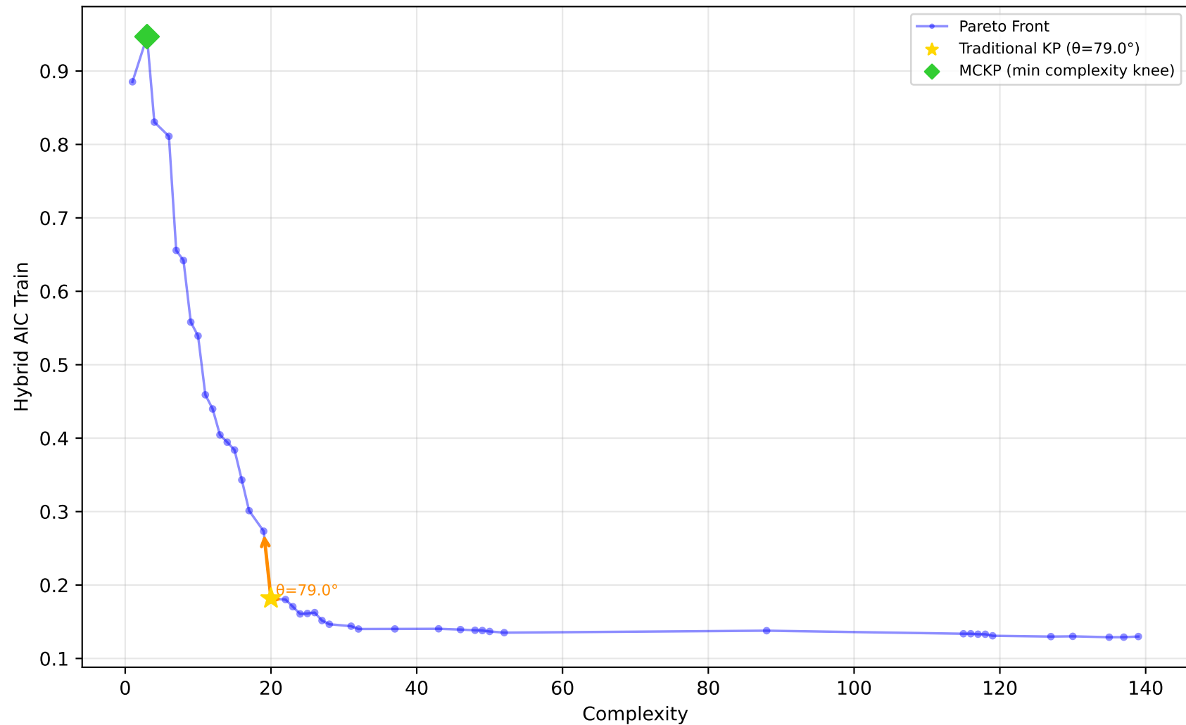
227_cpu_small - Run 7 - MVP - Hybrid AIC Train \lambda_1=0.80, \bar{\lambda}_2=0.20, \lambda_3=0.00 | Difficulty: 1.00 | Method: hmr
