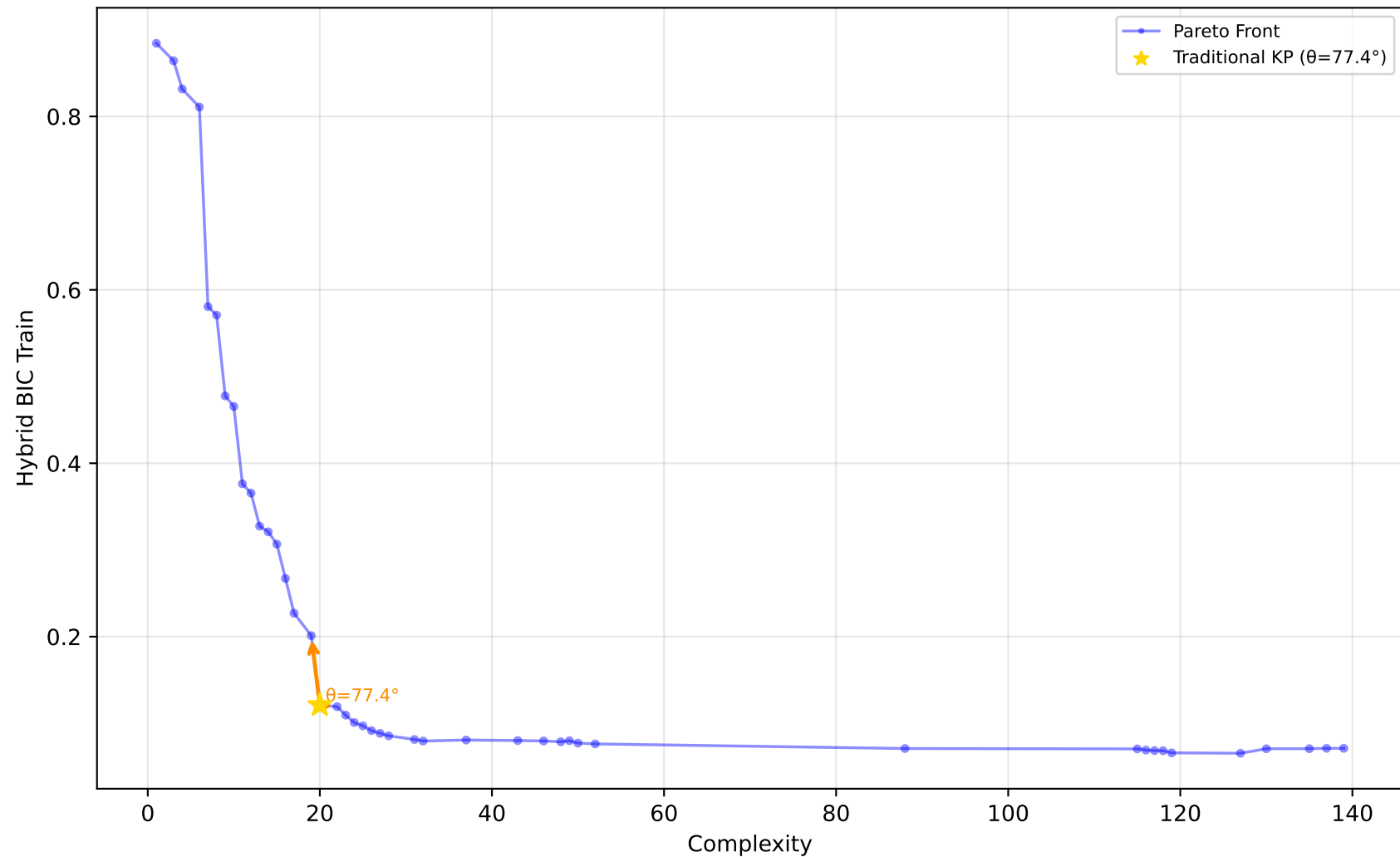
227_cpu_small - Run 7 - MVP - Hybrid BIC Train \lambda_1=0.00, \bar{\lambda}_2=0.90, \lambda_3=0.10 | Difficulty: 1.00 | Method: hmr
