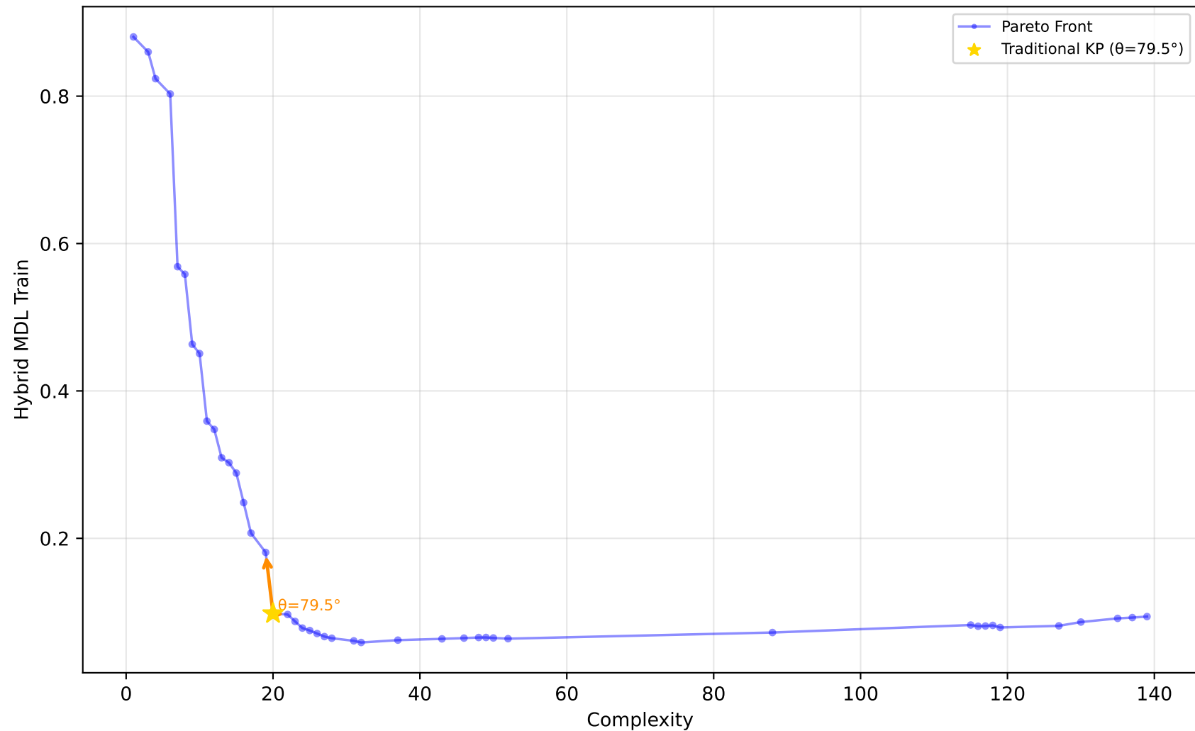
227_cpu_small - Run 7 - MVP - Hybrid MDL Train \lambda_1=0.00, \bar{\lambda}_2=0.90, \lambda_3=0.10 | Difficulty: 1.00 | Method: hmr
