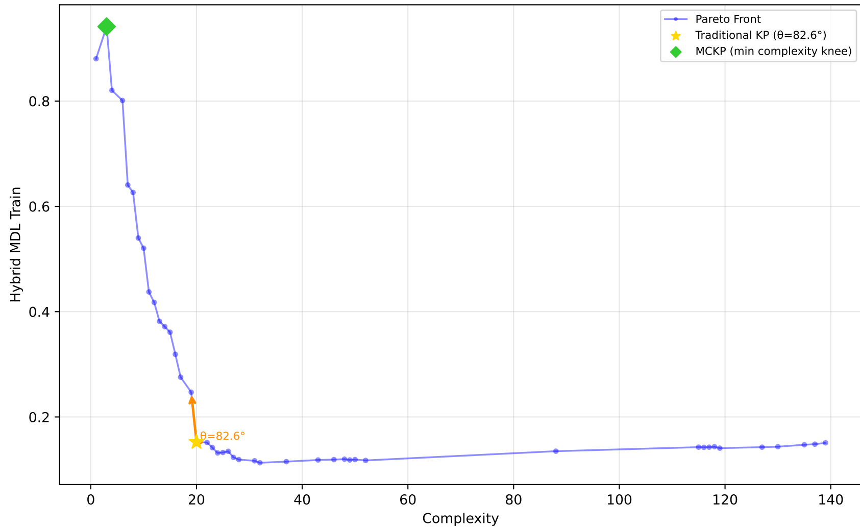
227_cpu_small - Run 7 - MVP - Hybrid MDL Train \lambda_1=0.80, \bar{\lambda}_2=0.20, \lambda_3=0.00 | Difficulty: 1.00 | Method: hmr
