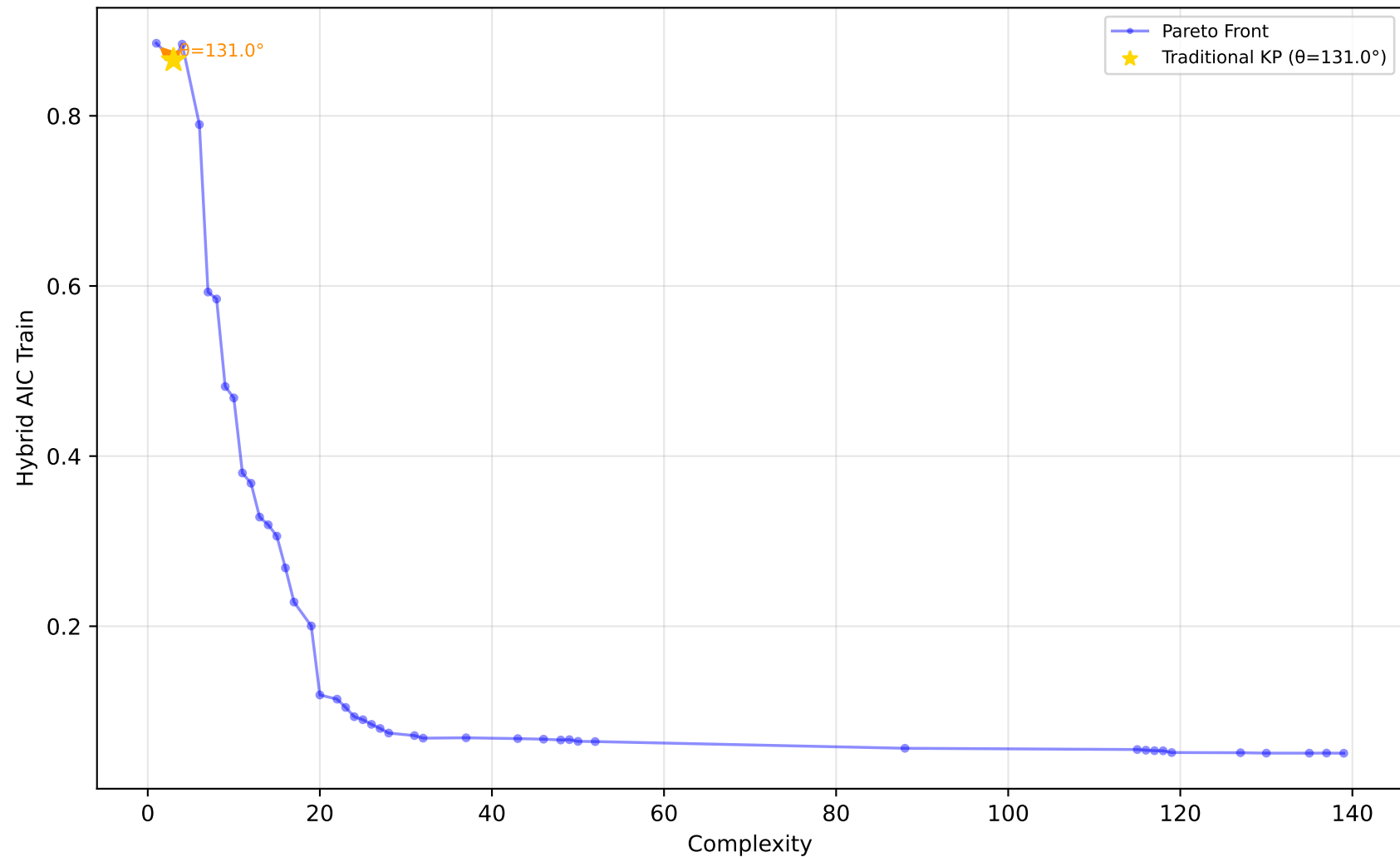
227_cpu_small - Run 7 - SVP - Hybrid AIC Train \lambda_1=0.00, \lambda_2=0.80, \lambda_3=0.30 | Difficulty: 1.00 | Method: hmr
