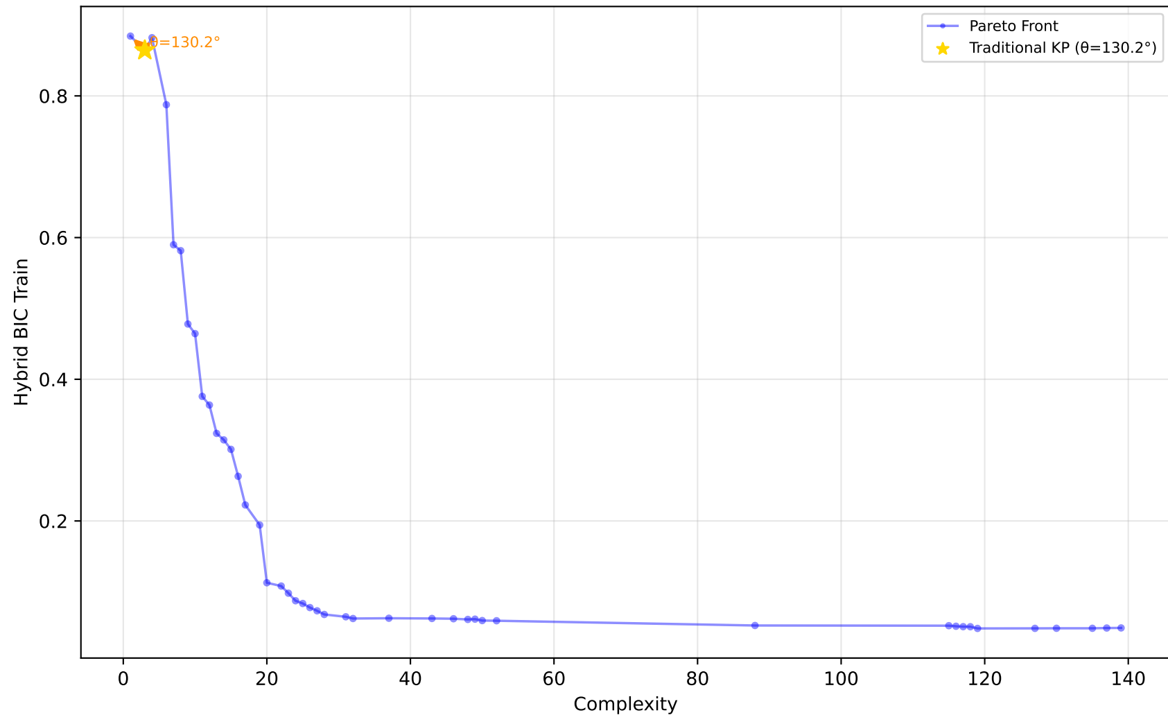
227_cpu_small - Run 7 - SVP - Hybrid BIC Train \lambda_1=0.00, \lambda_2=0.80, \lambda_3=0.30 | Difficulty: 1.00 | Method: hmr
