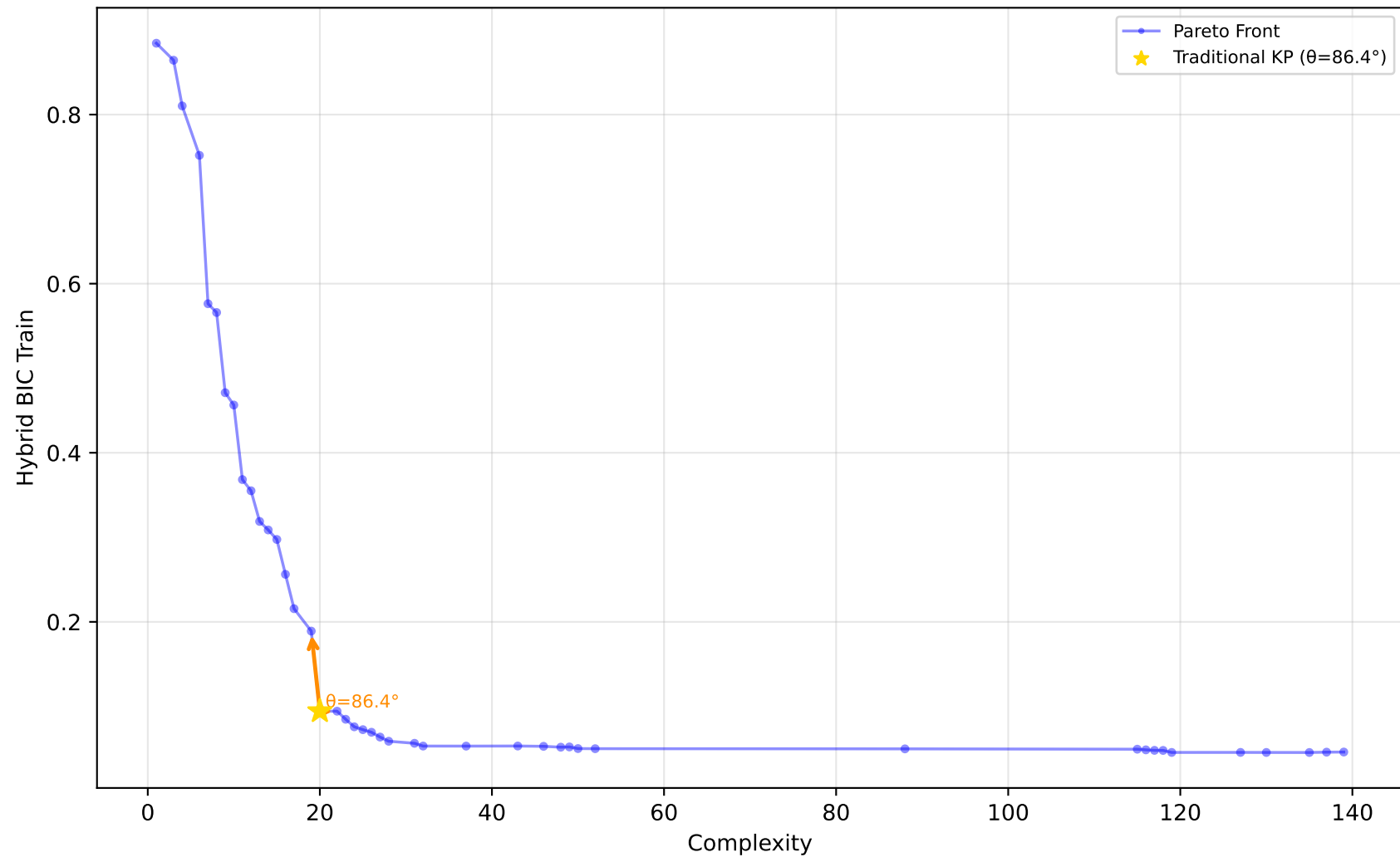
227_cpu_small - Run 7 - SVP - Hybrid BIC Train \lambda_1=0.00, \bar{\lambda}_2=1.00, \lambda_3=0.00 | Difficulty: 1.00 | Method: hmr
