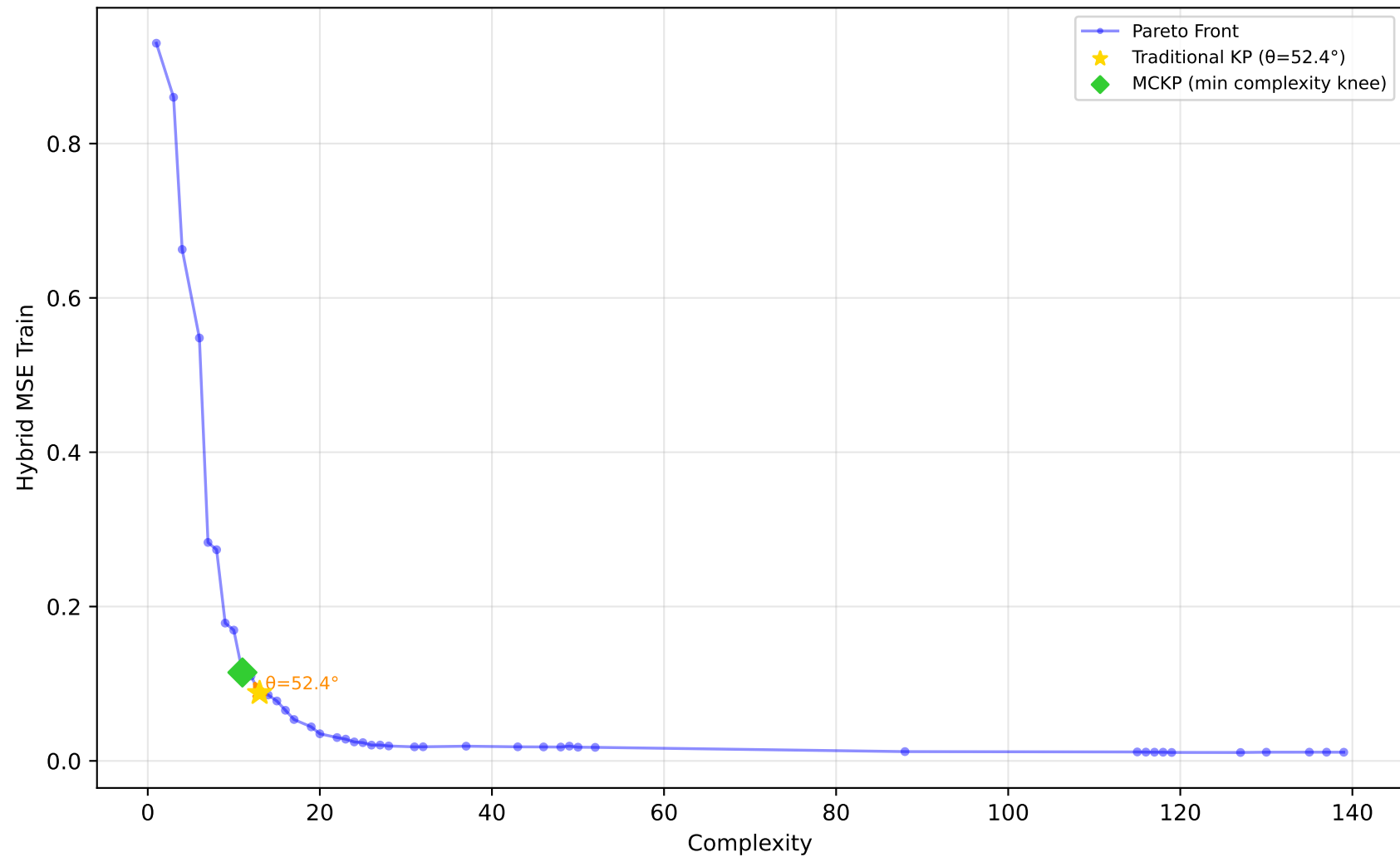
227_cpu_small - Run 7 - SVP - Hybrid MSE Train \lambda_1=0.00, \bar{\lambda}_2=0.80, \lambda_3=0.30 | Difficulty: 1.00 | Method: hmr
