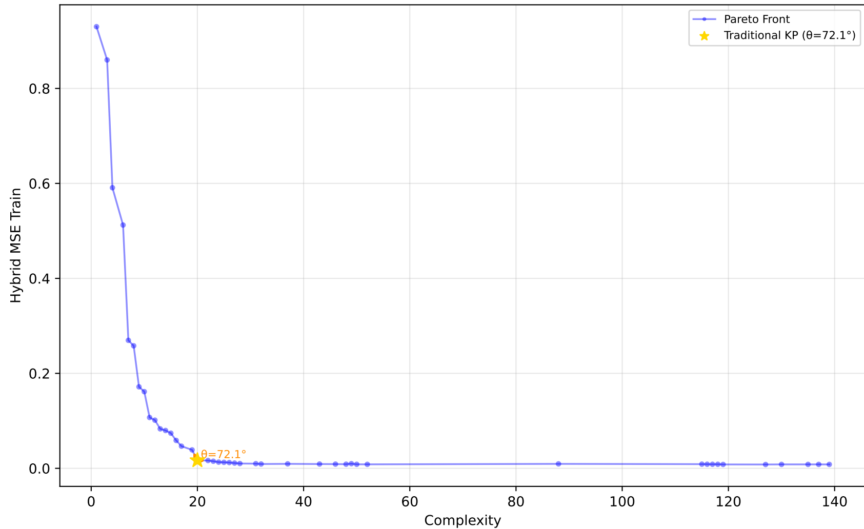
227_cpu_small - Run 7 - SVP - Hybrid MSE Train \lambda_1=0.00, \lambda_2=1.00, \lambda_3=0.00 | Difficulty: 1.00 | Method: hmr
