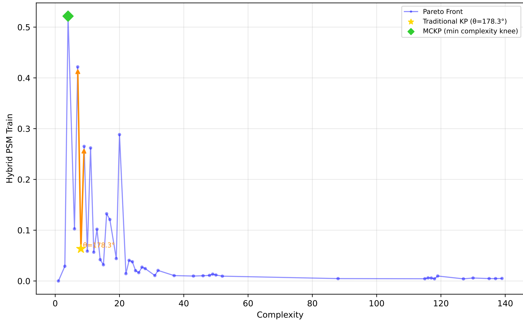
227_cpu_small - Run 7 - SVP - Hybrid PSM Train \lambda_1=0.00, \bar{\lambda}_2=0.80, \lambda_3=0.30 | Difficulty: 1.00 | Method: hmr
