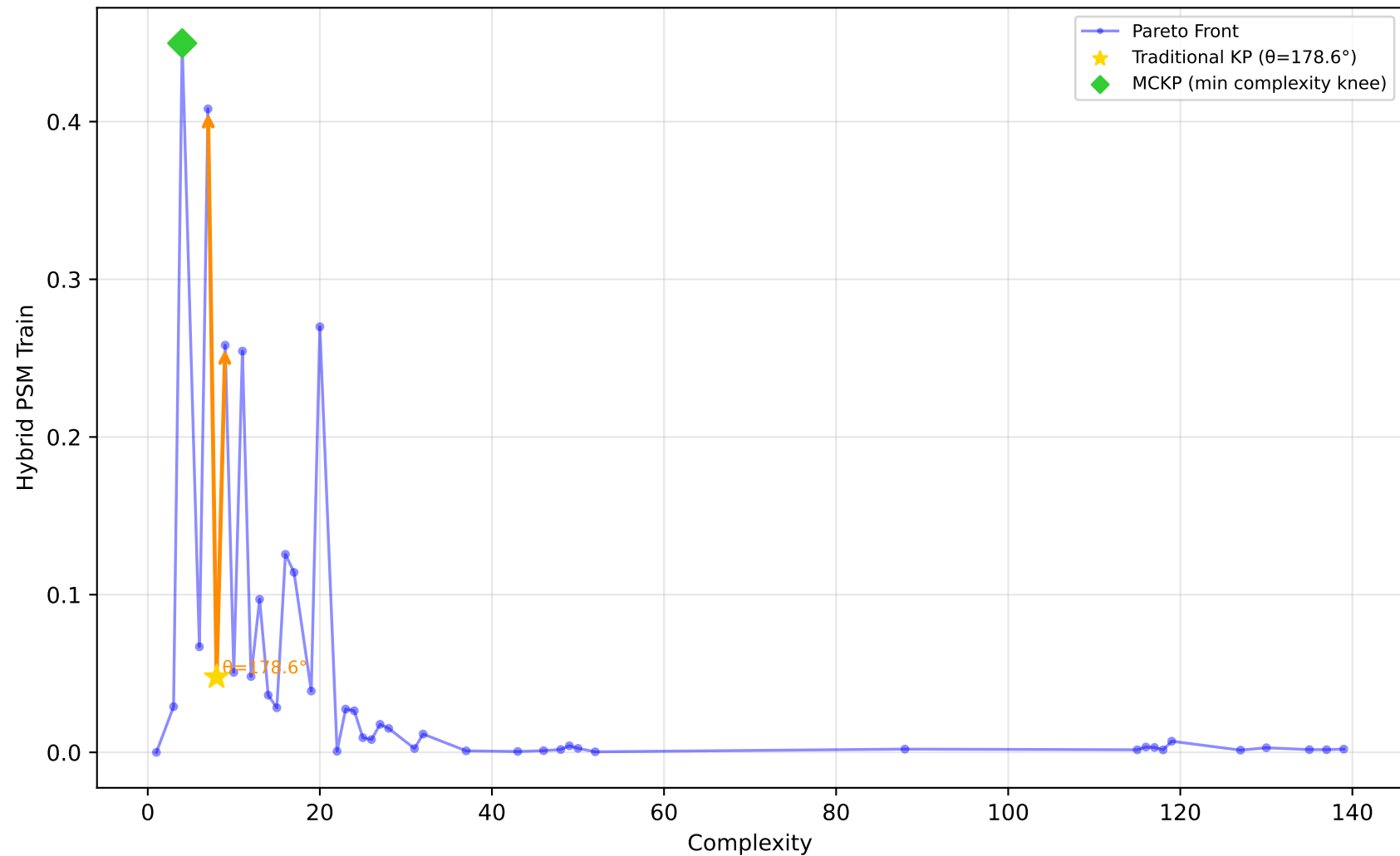
227_cpu_small - Run 7 - SVP - Hybrid PSM Train \lambda_1=0.00, \lambda_2=1.00, \lambda_3=0.00 | Difficulty: 1.00 | Method: hmr
