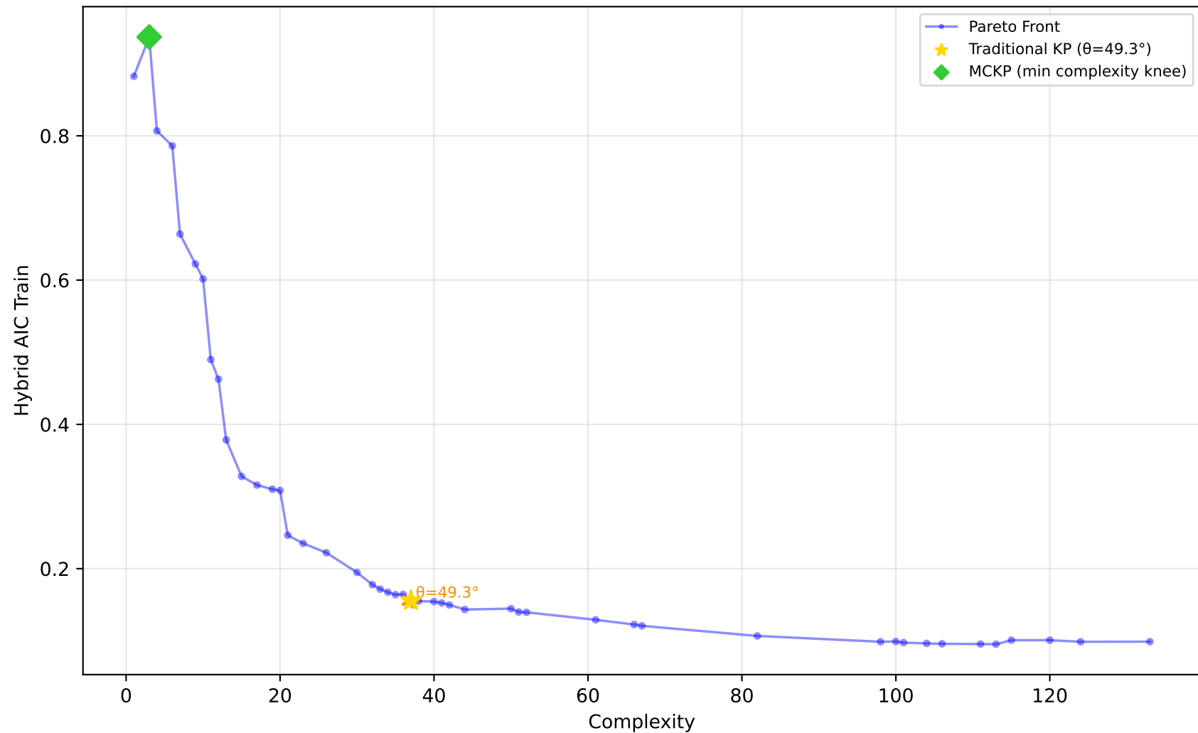
227_cpu_small - Run 8 - MVP - Hybrid AIC Train \lambda_1=0.80, \bar{\lambda}_2=0.20, \lambda_3=0.00 | Difficulty: 1.00 | Method: hmr
