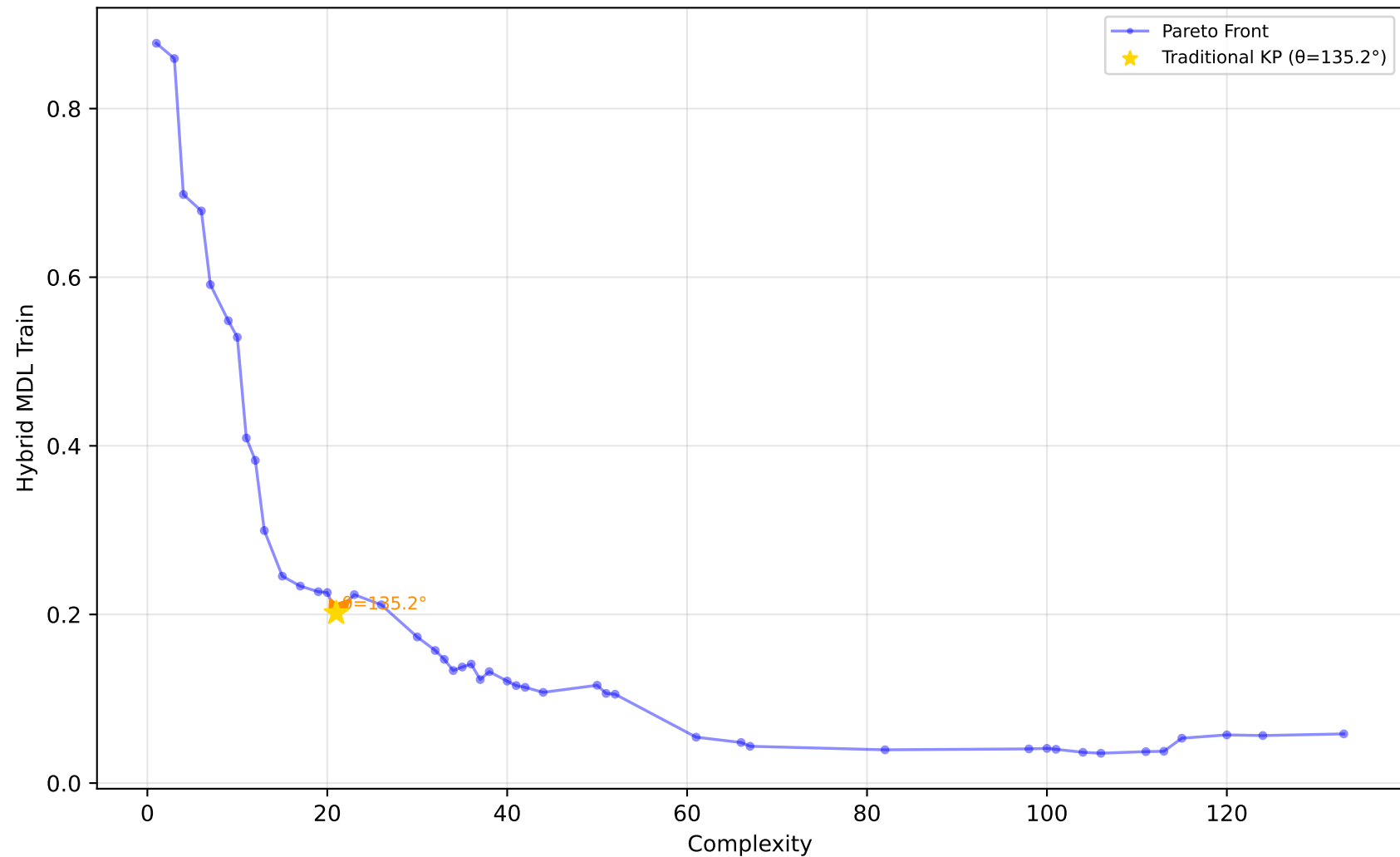
227_cpu_small - Run 8 - MVP - Hybrid MDL Train \lambda_1=0.00, \bar{\lambda}_2=0.90, \lambda_3=0.10 | Difficulty: 1.00 | Method: hmr
