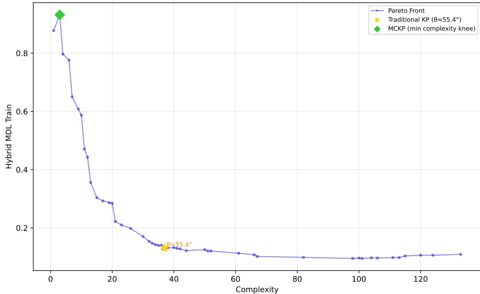
227_cpu_small - Run 8 - MVP - Hybrid MDL Train \lambda_1=0.80, \bar{\lambda}_2=0.20, \lambda_3=0.00 | Difficulty: 1.00 | Method: hmr
