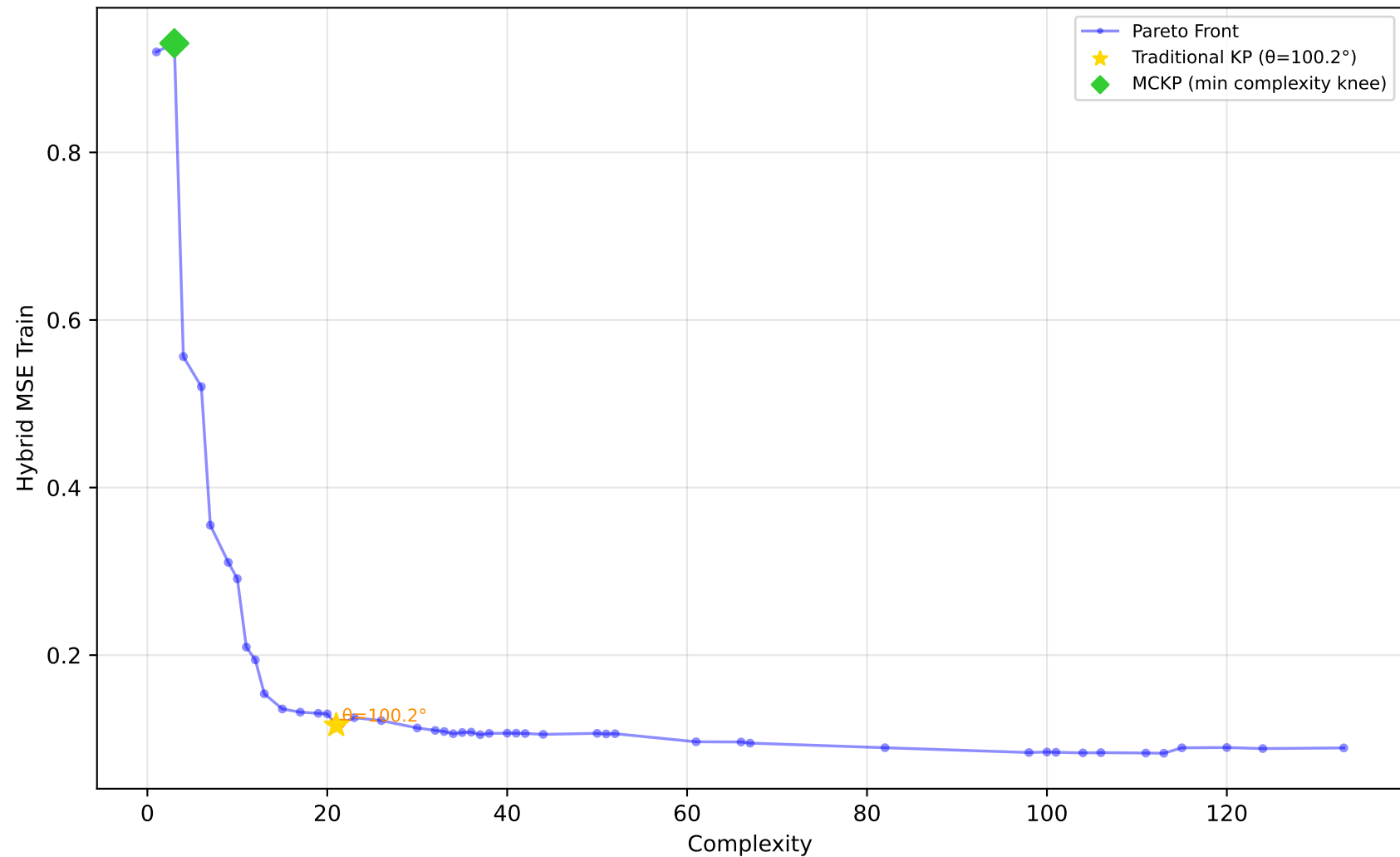
227_cpu_small - Run 8 - MVP - Hybrid MSE Train \lambda_1=0.80, \bar{\lambda}_2=0.20, \lambda_3=0.00 | Difficulty: 1.00 | Method: hmr
