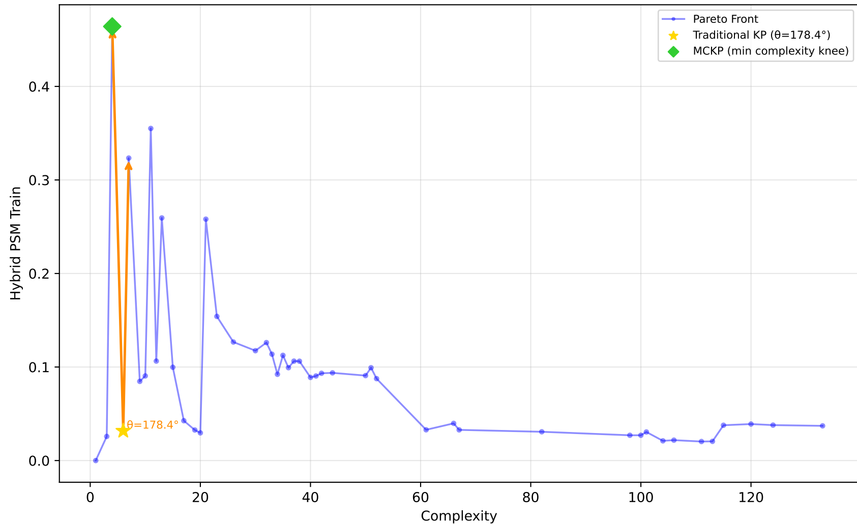
227_cpu_small - Run 8 - MVP - Hybrid PSM Train \lambda_1=0.00, \bar{\lambda}_2=0.90, \lambda_3=0.10 | Difficulty: 1.00 | Method: hmr
