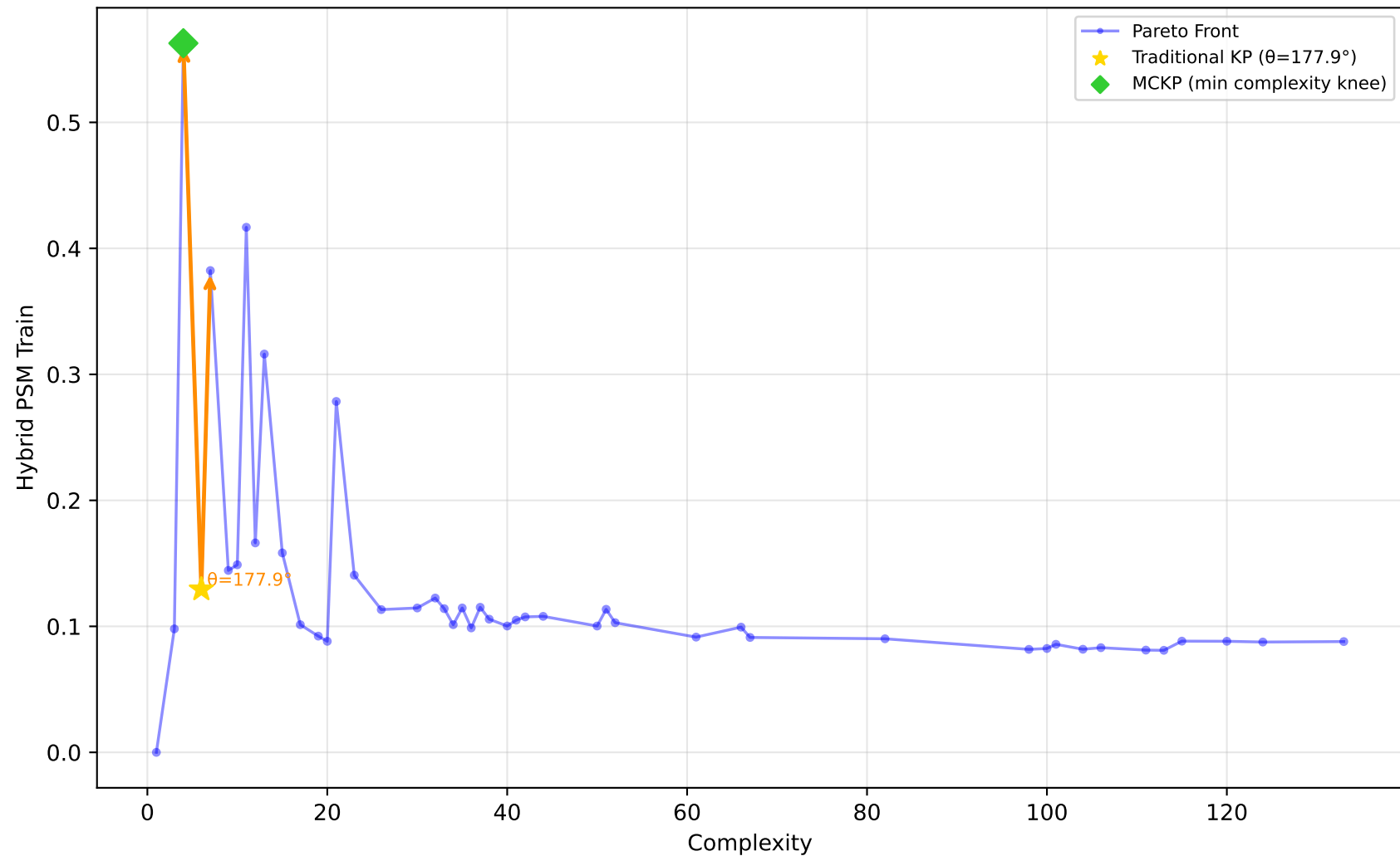
227_cpu_small - Run 8 - MVP - Hybrid PSM Train \lambda_1=0.80, \bar{\lambda}_2=0.20, \lambda_3=0.00 | Difficulty: 1.00 | Method: hmr
