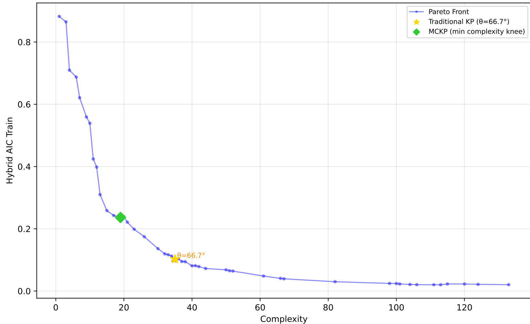
227_cpu_small - Run 8 - SVP - Hybrid AIC Train \lambda_1=0.00, \bar{\lambda}_2=0.80, \lambda_3=0.30 | Difficulty: 1.00 | Method: hmr
