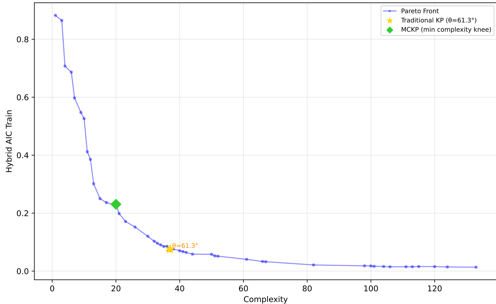
227_cpu_small - Run 8 - SVP - Hybrid AIC Train \lambda_1=0.00, \bar{\lambda}_2=1.00, \lambda_3=0.00 | Difficulty: 1.00 | Method: hmr
