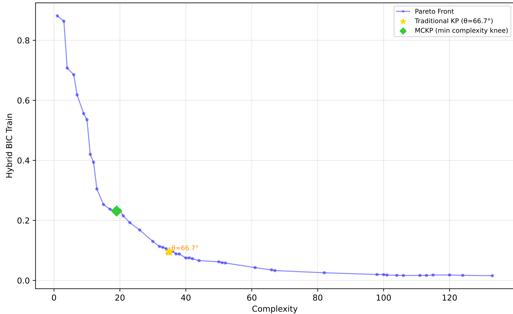
227_cpu_small - Run 8 - SVP - Hybrid BIC Train \lambda_1=0.00, \bar{\lambda}_2=0.80, \lambda_3=0.30 | Difficulty: 1.00 | Method: hmr
