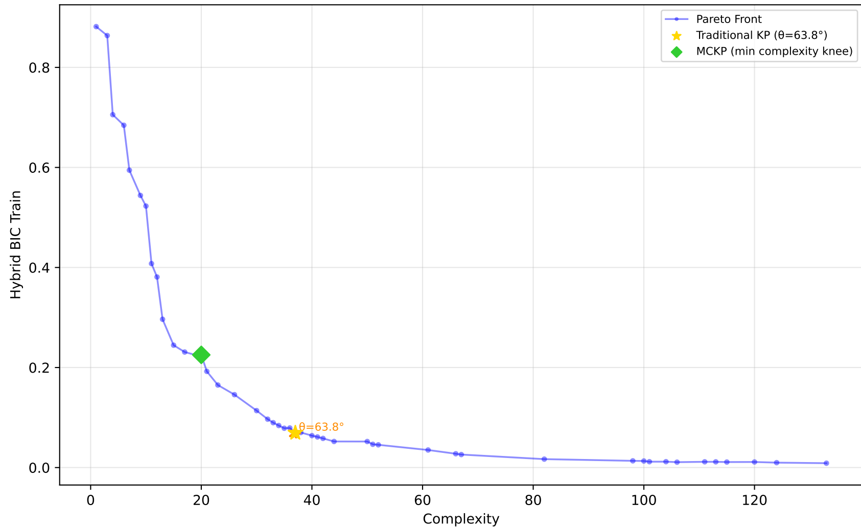
227_cpu_small - Run 8 - SVP - Hybrid BIC Train \lambda_1=0.00, \bar{\lambda}_2=1.00, \lambda_3=0.00 | Difficulty: 1.00 | Method: hmr
