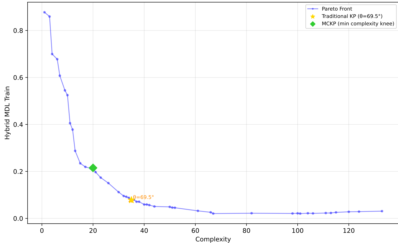
227_cpu_small - Run 8 - SVP - Hybrid MDL Train \lambda_1=0.00, \bar{\lambda}_2=0.80, \lambda_3=0.30 | Difficulty: 1.00 | Method: hmr
