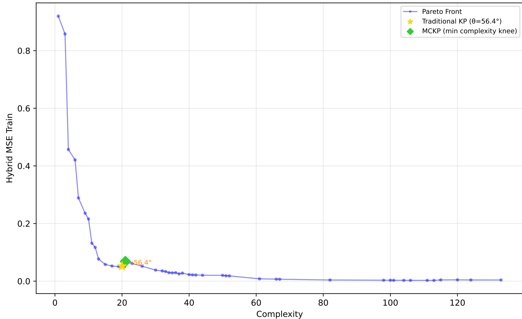
227_cpu_small - Run 8 - SVP - Hybrid MSE Train \lambda_1=0.00, \lambda_2=1.00, \lambda_3=0.00 | Difficulty: 1.00 | Method: hmr
