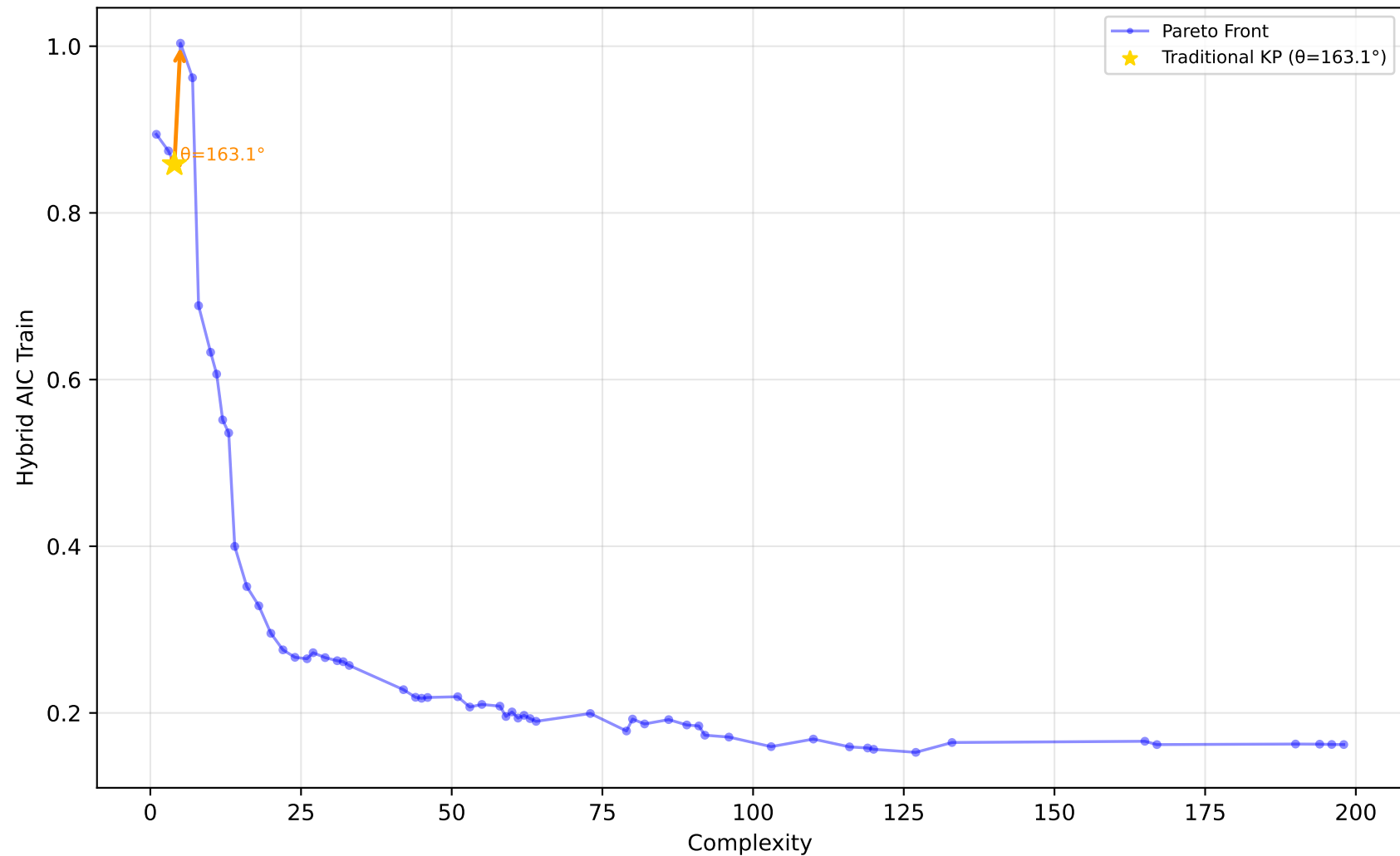
227_cpu_small - Run 9 - MVP - Hybrid AIC Train \lambda_1=0.00, \bar{\lambda}_2=0.90, \lambda_3=0.10 | Difficulty: 1.00 | Method: hmr
