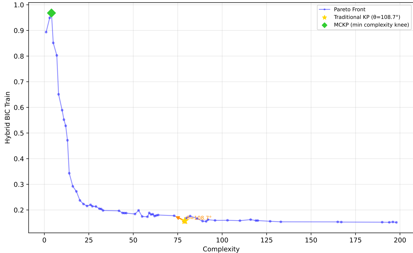
227_cpu_small - Run 9 - MVP - Hybrid BIC Train \lambda_1=0.80, \bar{\lambda}_2=0.20, \lambda_3=0.00 | Difficulty: 1.00 | Method: hmr
