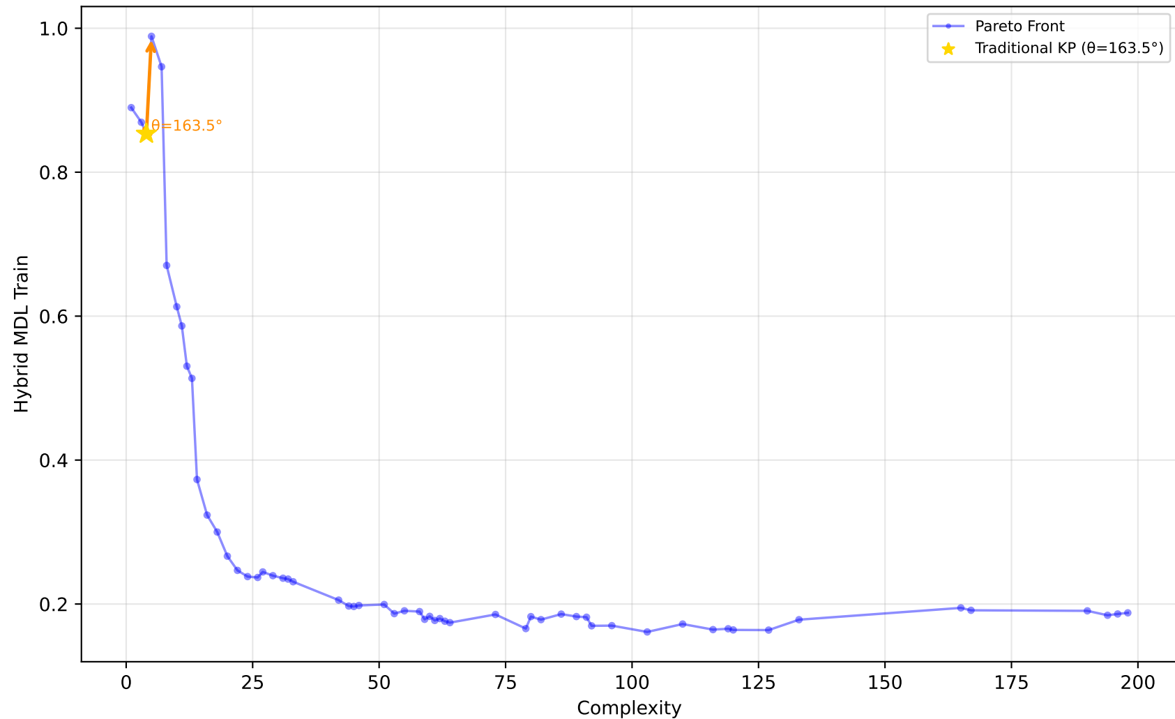
227_cpu_small - Run 9 - MVP - Hybrid MDL Train \lambda_1=0.00, \bar{\lambda}_2=0.90, \lambda_3=0.10 | Difficulty: 1.00 | Method: hmr
