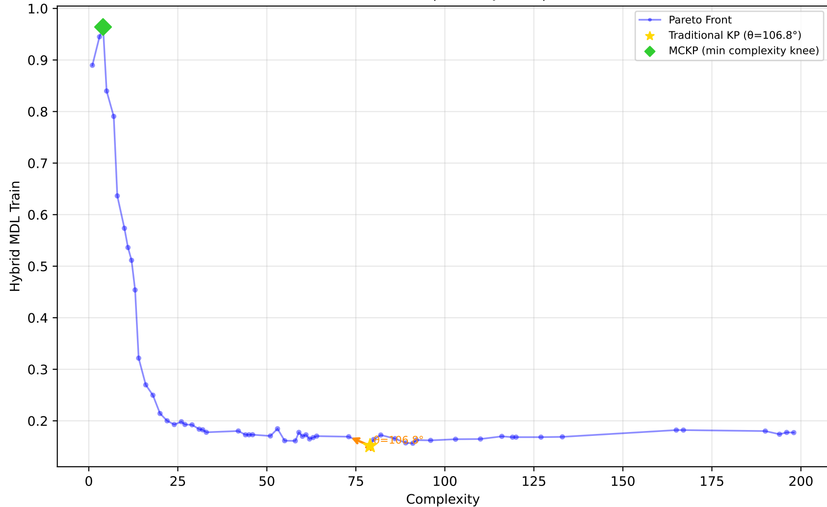
227_cpu_small - Run 9 - MVP - Hybrid MDL Train \lambda_1=0.80, \bar{\lambda}_2=0.20, \lambda_3=0.00 | Difficulty: 1.00 | Method: hmr
