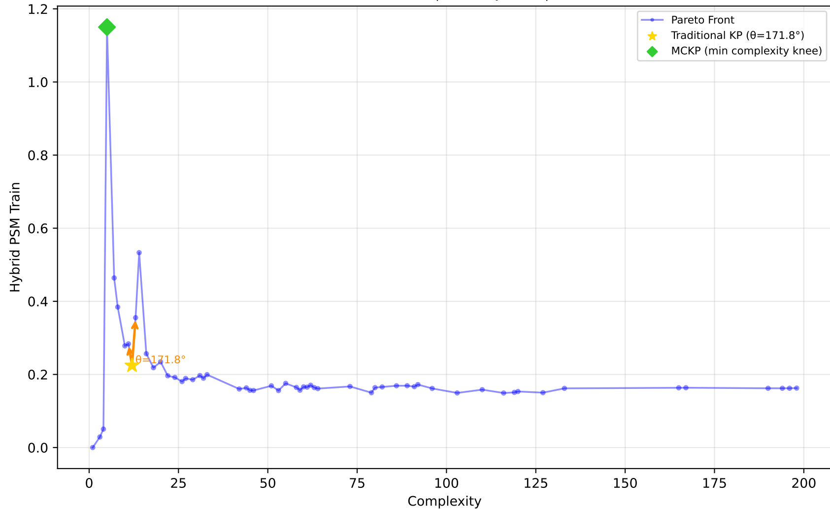
227_cpu_small - Run 9 - MVP - Hybrid PSM Train \lambda_1=0.00, \bar{\lambda}_2=0.90, \lambda_3=0.10 | Difficulty: 1.00 | Method: hmr
