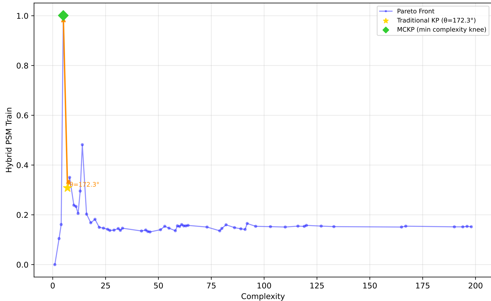
227_cpu_small - Run 9 - MVP - Hybrid PSM Train \lambda_1=0.80, \bar{\lambda}_2=0.20, \lambda_3=0.00 | Difficulty: 1.00 | Method: hmr
