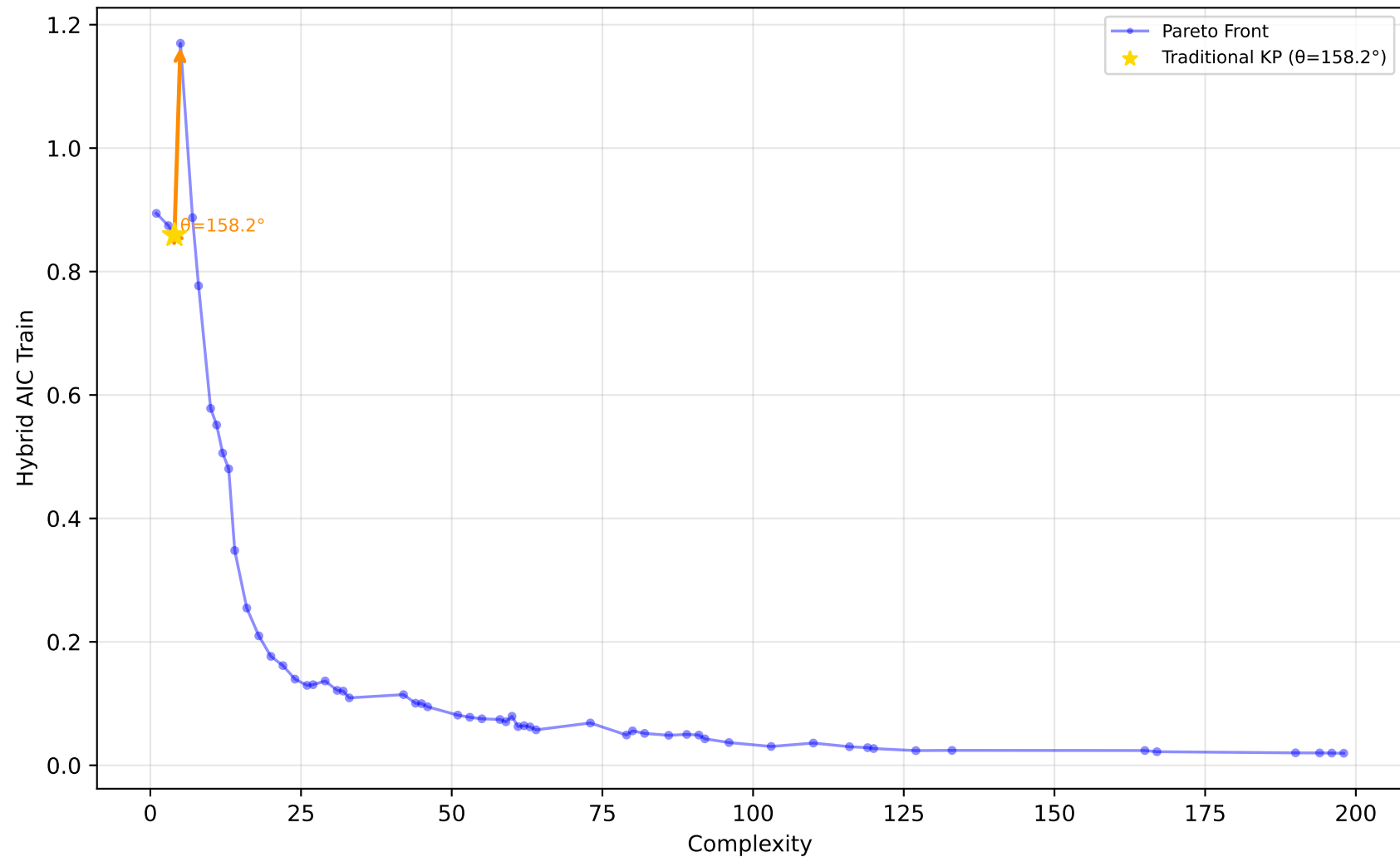
227_cpu_small - Run 9 - SVP - Hybrid AIC Train \lambda_1=0.00, \bar{\lambda}_2=0.80, \lambda_3=0.30 | Difficulty: 1.00 | Method: hmr
