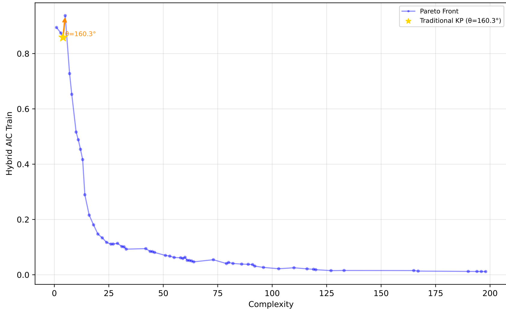
227_cpu_small - Run 9 - SVP - Hybrid AIC Train \lambda_1=0.00, \lambda_2=1.00, \lambda_3=0.00 | Difficulty: 1.00 | Method: hmr
