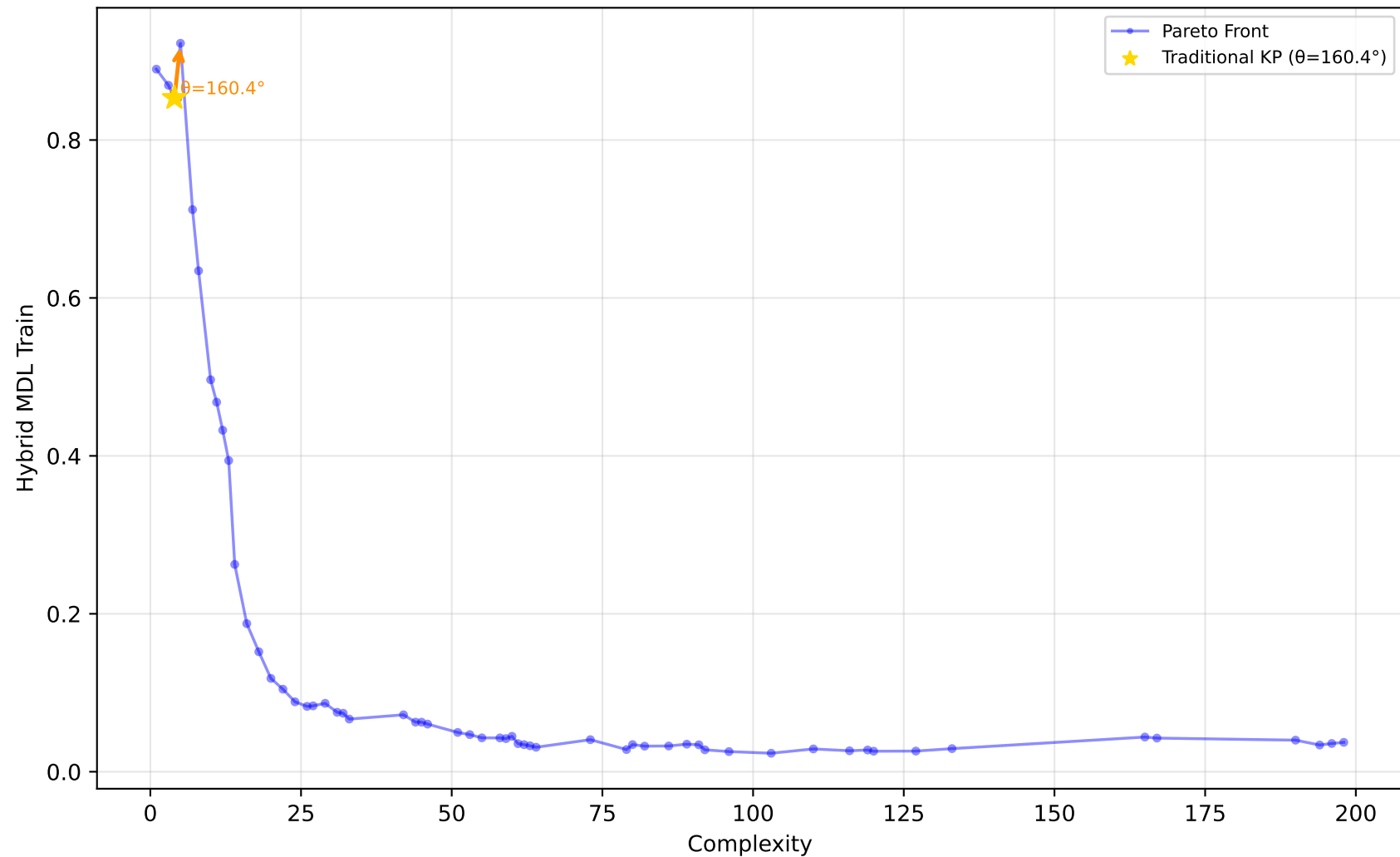
227_cpu_small - Run 9 - SVP - Hybrid MDL Train \lambda_1=0.00, \lambda_2=1.00, \lambda_3=0.00 | Difficulty: 1.00 | Method: hmr
