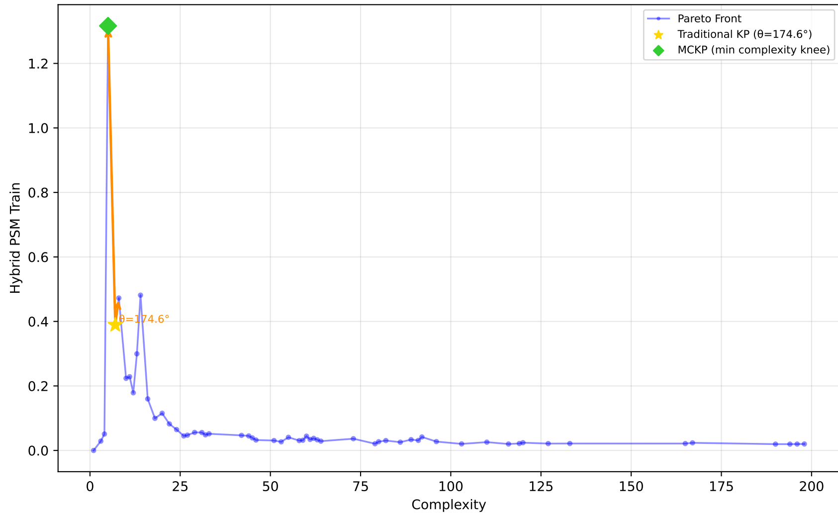
227_cpu_small - Run 9 - SVP - Hybrid PSM Train \lambda_1=0.00, \lambda_2=0.80, \lambda_3=0.30 | Difficulty: 1.00 | Method: hmr
