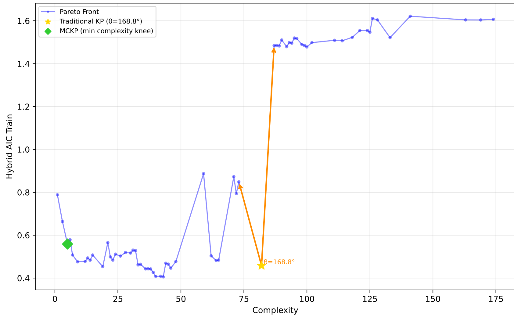
192_vineyard - Run 10 - MVP - Hybrid AIC Train \lambda_1=0.00, \lambda_2=0.30, \lambda_3=1.00 | Difficulty: 0.17 | Method: mckp
