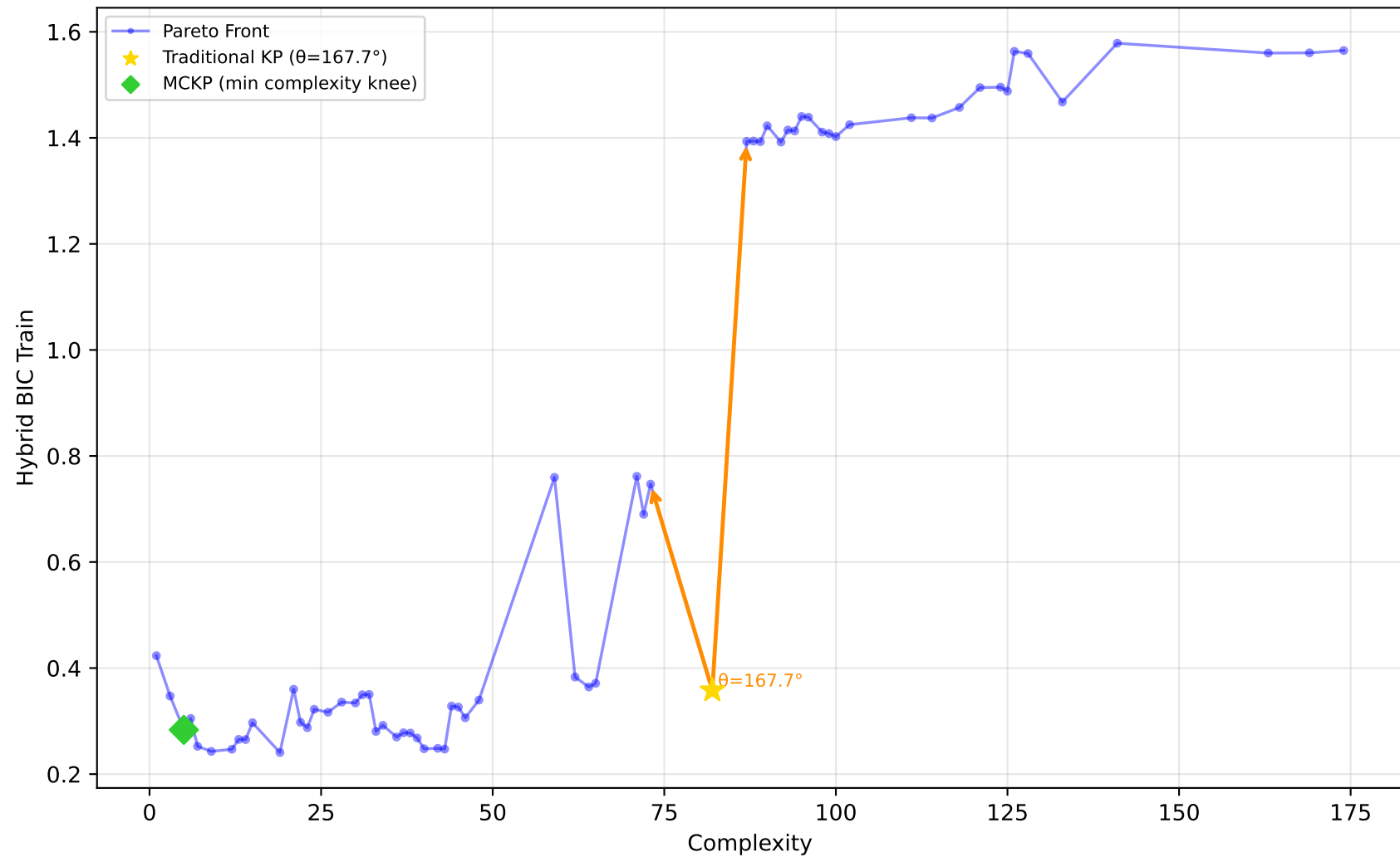
192_vineyard - Run 10 - MVP - Hybrid BIC Train \lambda_1=0.00, \lambda_2=0.30, \lambda_3=1.00 | Difficulty: 0.17 | Method: mckp
