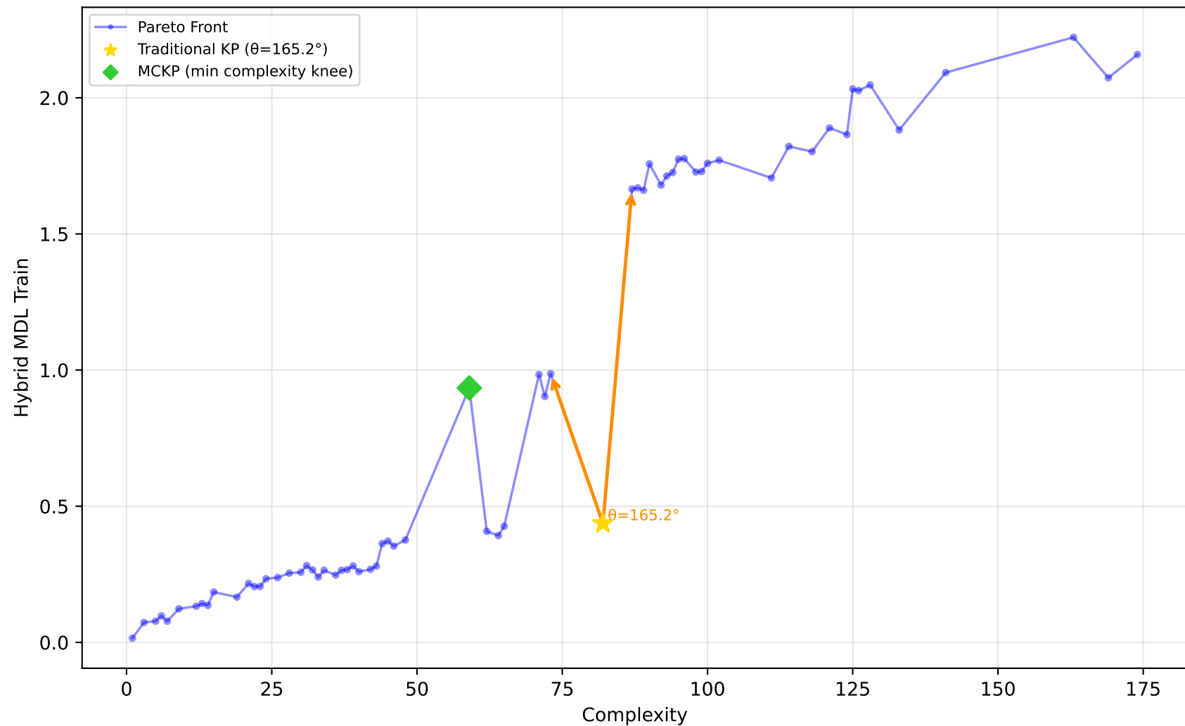
192_vineyard - Run 10 - MVP - Hybrid MDL Train \lambda_1=0.40, \bar{\lambda}_2=0.00, \lambda_3=1.00 | Difficulty: 0.17 | Method: mckp
