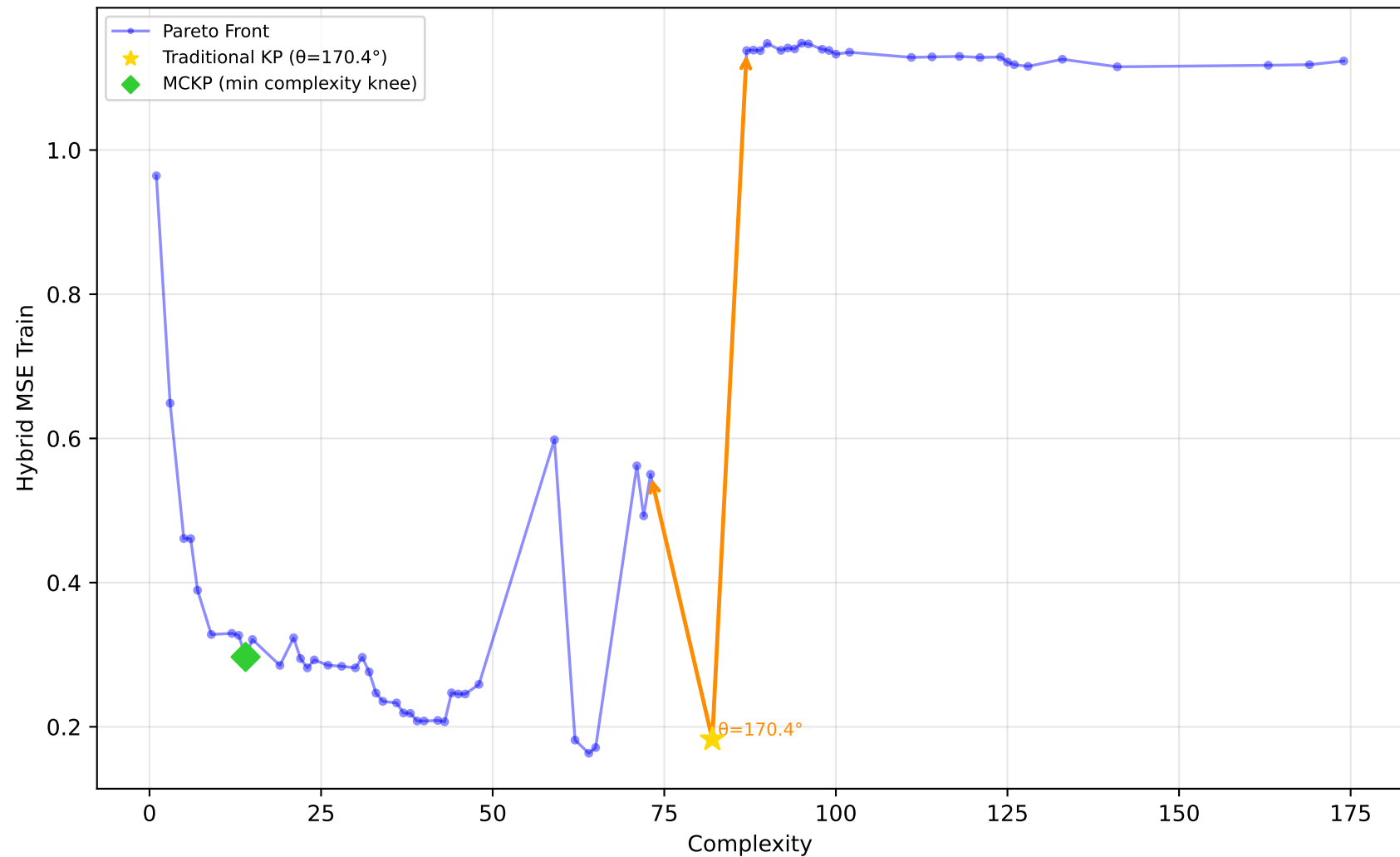
192_vineyard - Run 10 - MVP - Hybrid MSE Train \lambda_1=0.00, \bar{\lambda}_2=0.30, \lambda_3=1.00 | Difficulty: 0.17 | Method: mckp
