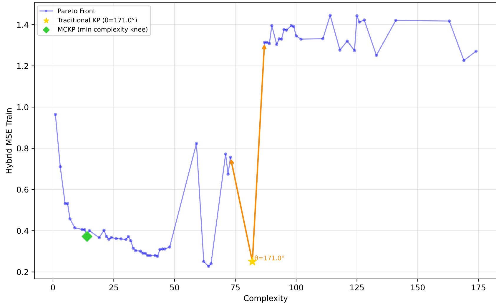
192_vineyard - Run 10 - MVP - Hybrid MSE Train \lambda_1=0.40, \lambda_2=0.00, \lambda_3=1.00 | Difficulty: 0.17 | Method: mckp
