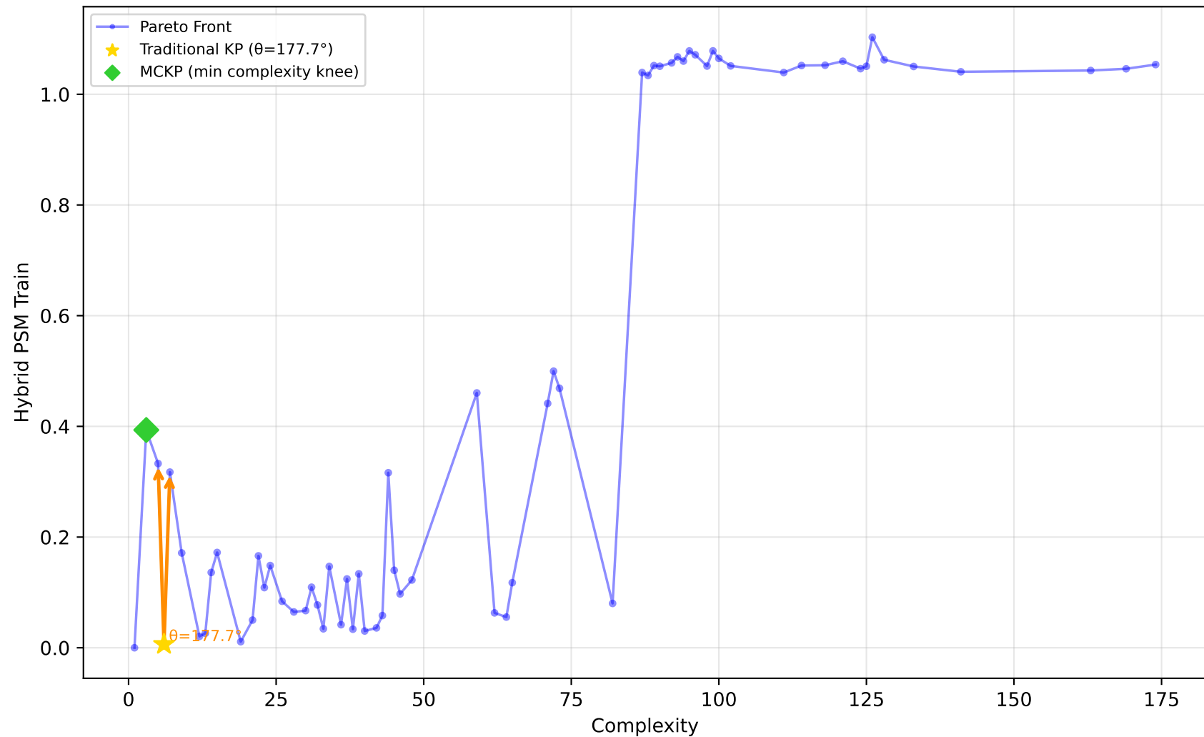
192_vineyard - Run 10 - MVP - Hybrid PSM Train \lambda_1=0.00, \lambda_2=0.30, \lambda_3=1.00 | Difficulty: 0.17 | Method: mckp
