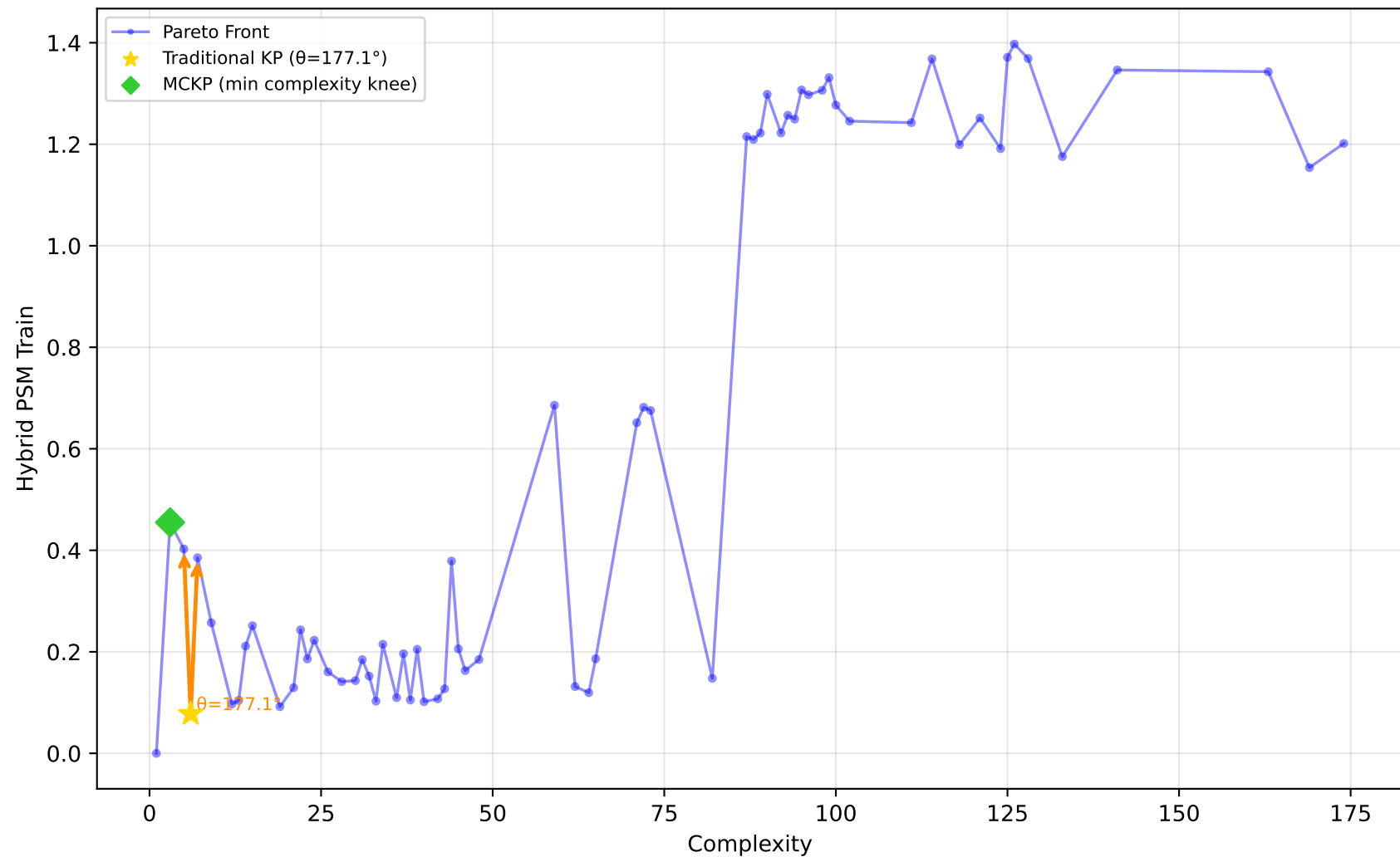
192_vineyard - Run 10 - MVP - Hybrid PSM Train \lambda_1=0.40, \bar{\lambda}_2=0.00, \lambda_3=1.00 | Difficulty: 0.17 | Method: mckp
