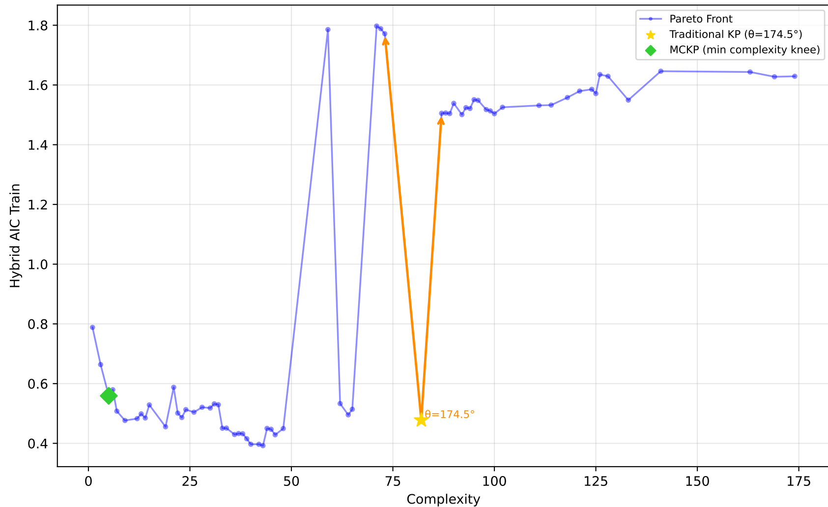
192_vineyard - Run 10 - SVP - Hybrid AIC Train \lambda_1=0.00, \lambda_2=1.00, \lambda_3=1.00 | Difficulty: 0.17 | Method: mckp
