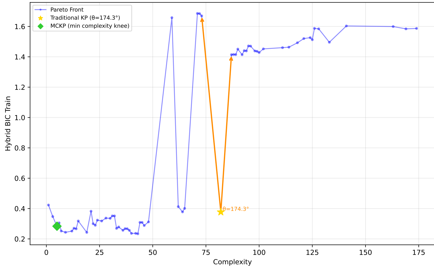
192_vineyard - Run 10 - SVP - Hybrid BIC Train \lambda_1=0.00, \lambda_2=1.00, \lambda_3=1.00 | Difficulty: 0.17 | Method: mckp
