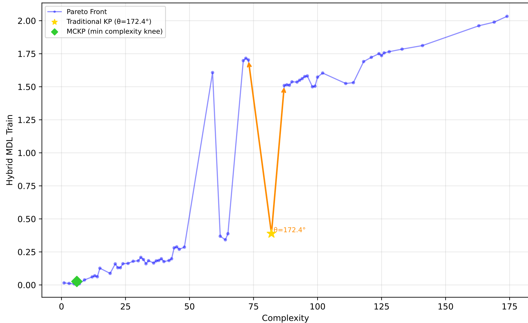
192_vineyard - Run 10 - SVP - Hybrid MDL Train \lambda_1=0.00, \lambda_2=1.00, \lambda_3=1.00 | Difficulty: 0.17 | Method: mckp
