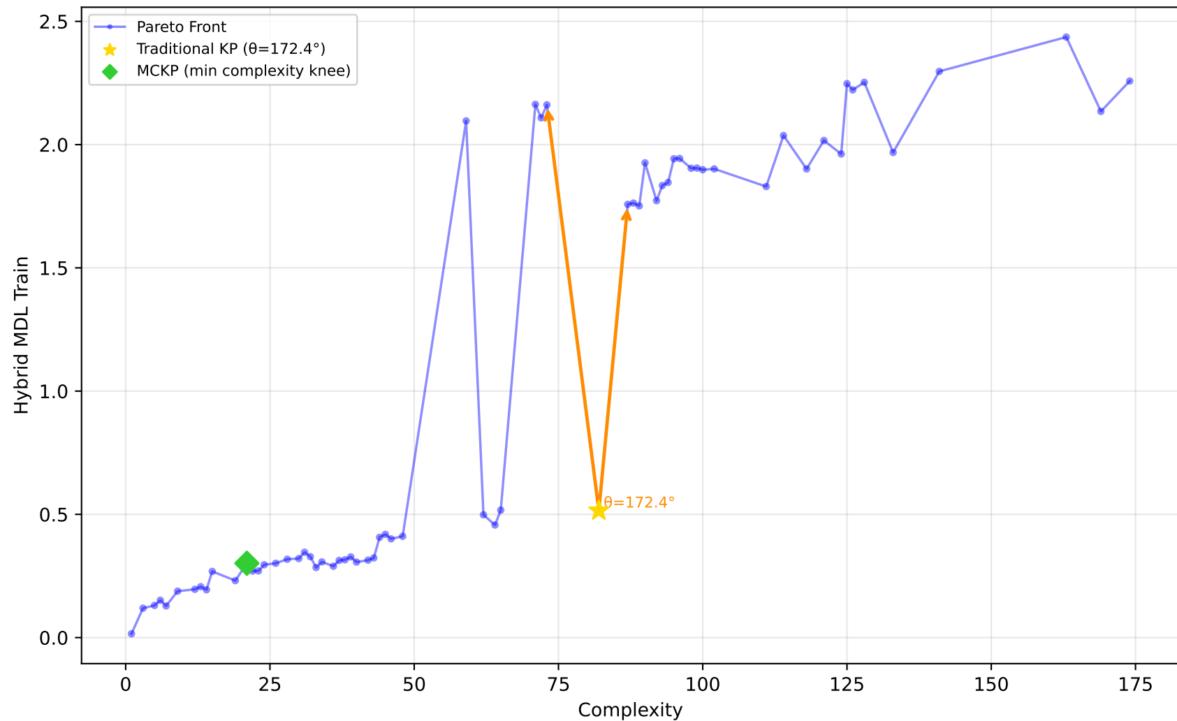
192_vineyard - Run 10 - SVP - Hybrid MDL Train \lambda_1=0.70, \lambda_2=0.70, \lambda_3=0.90 | Difficulty: 0.17 | Method: mckp
